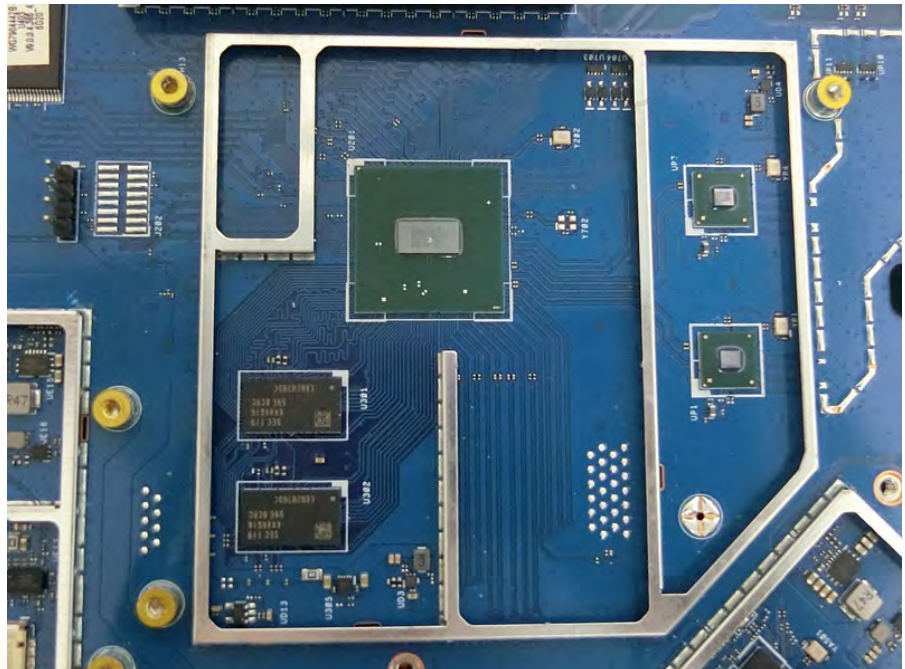
MLCC on the path of the CPU (Location: C124, C126, C127, C128) (Main Source)
