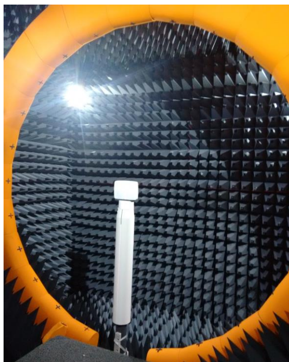
Figure 3、chamber
