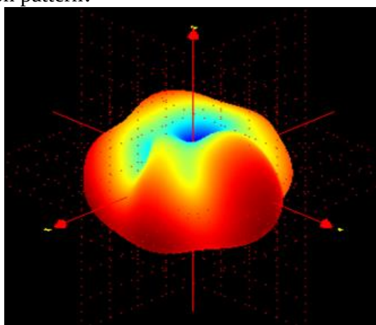
2.4GHz
