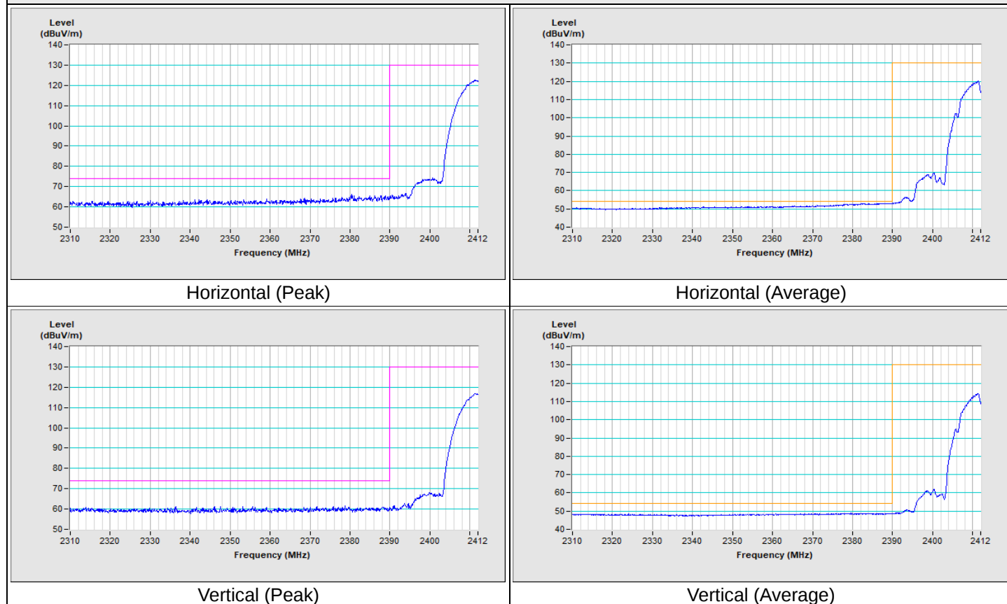
802.11b Channel 1
