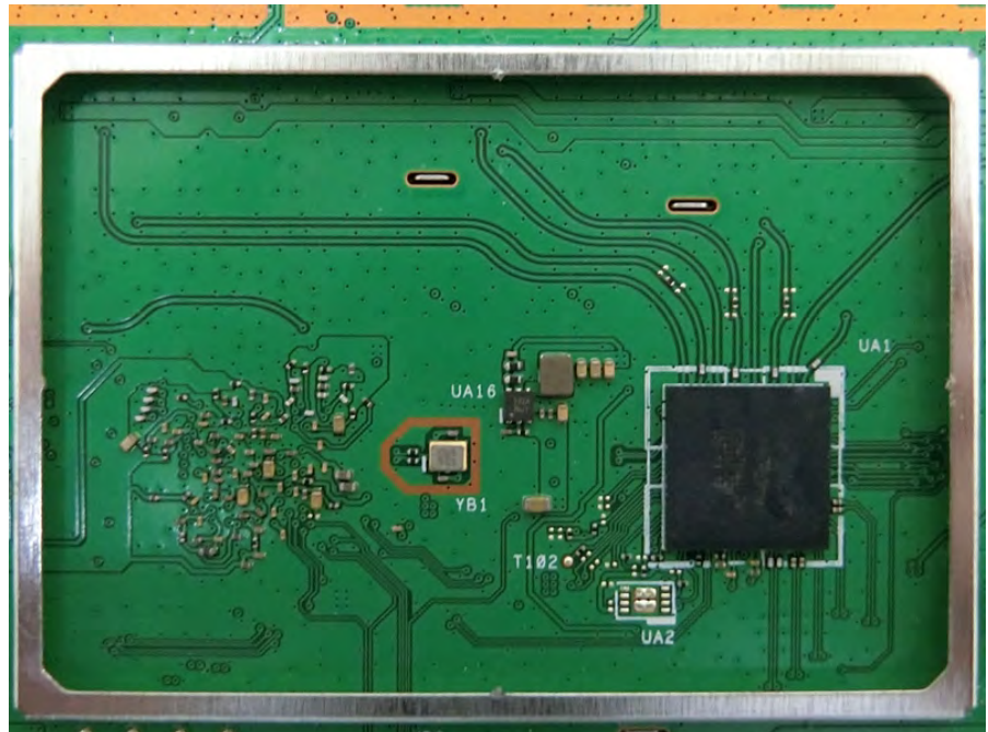
MLCC on the path of the CPU Second Source
