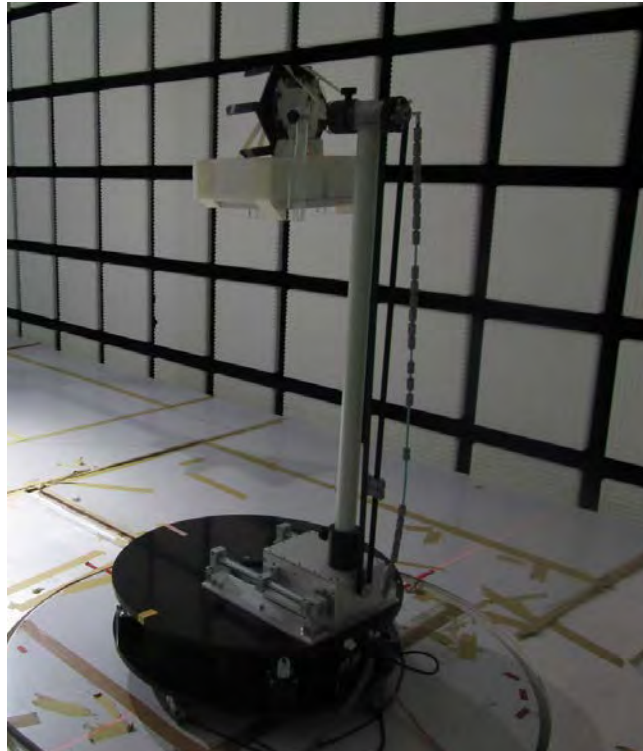
Test Setup Photos
