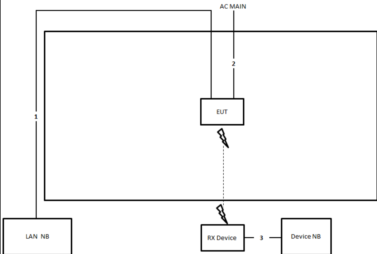
Test Setup Diagram - Radiated Test > 1GHz / For beamforming mode
