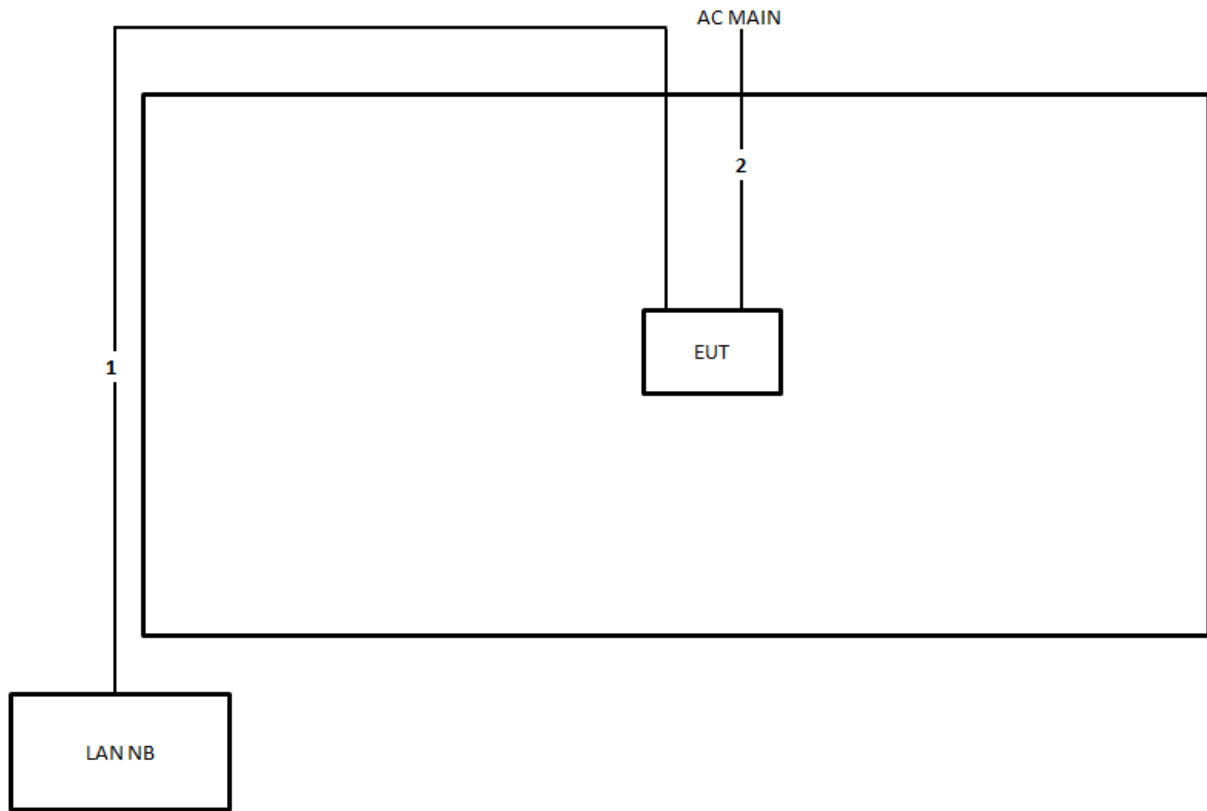
Test Setup Diagram - Radiated Test > 1GHz / For non-beamforming mode
