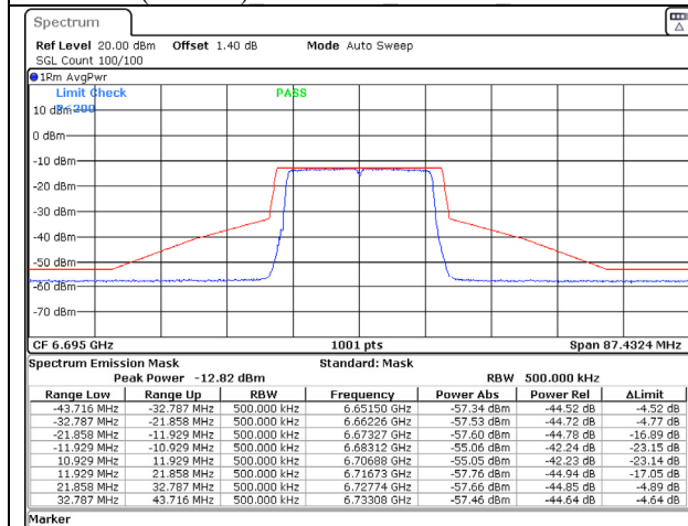
802.11ax (20MHz) 6695MHz Chain A NSS-2
