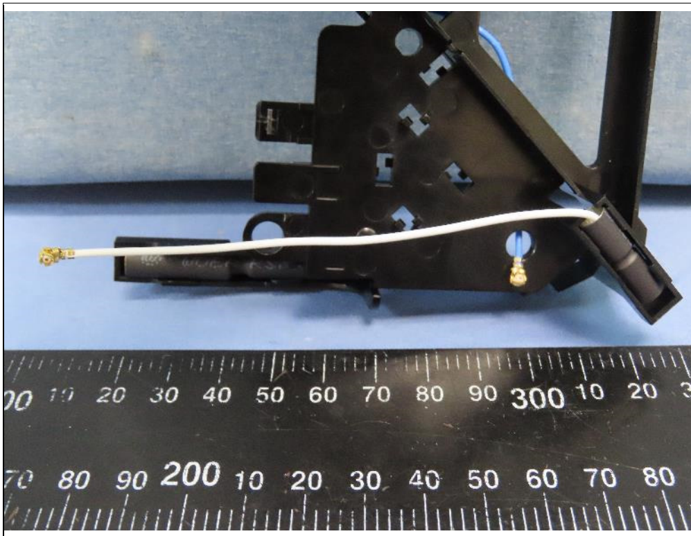
ANT_6G 1
