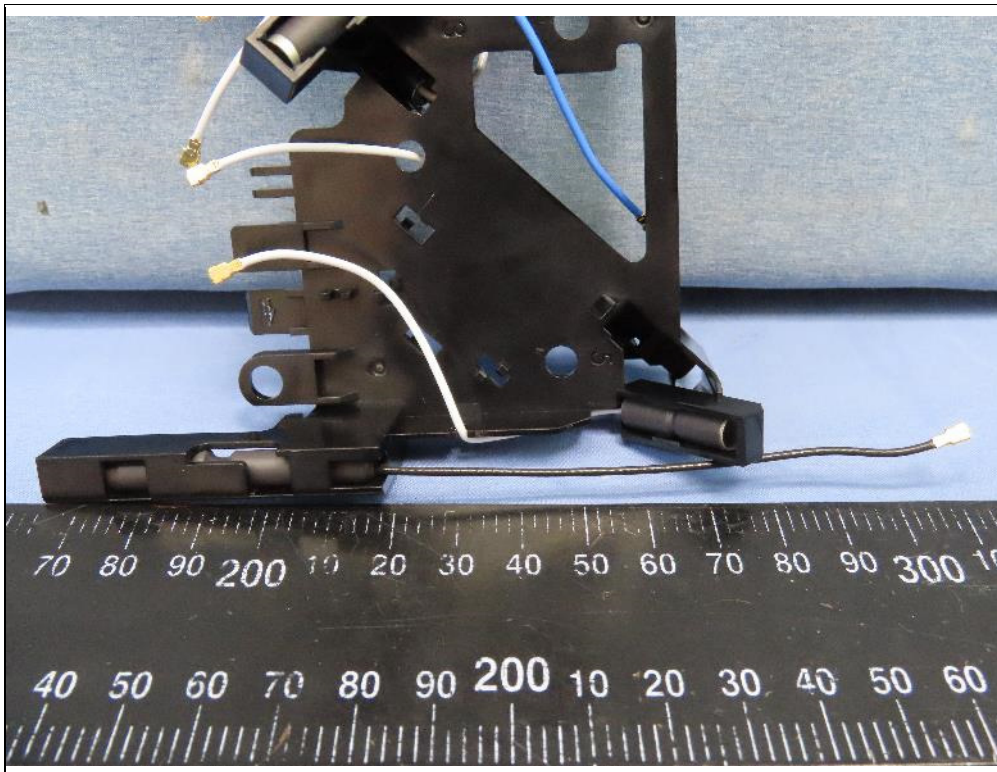
ANT_2.4G 1, 5G 1
