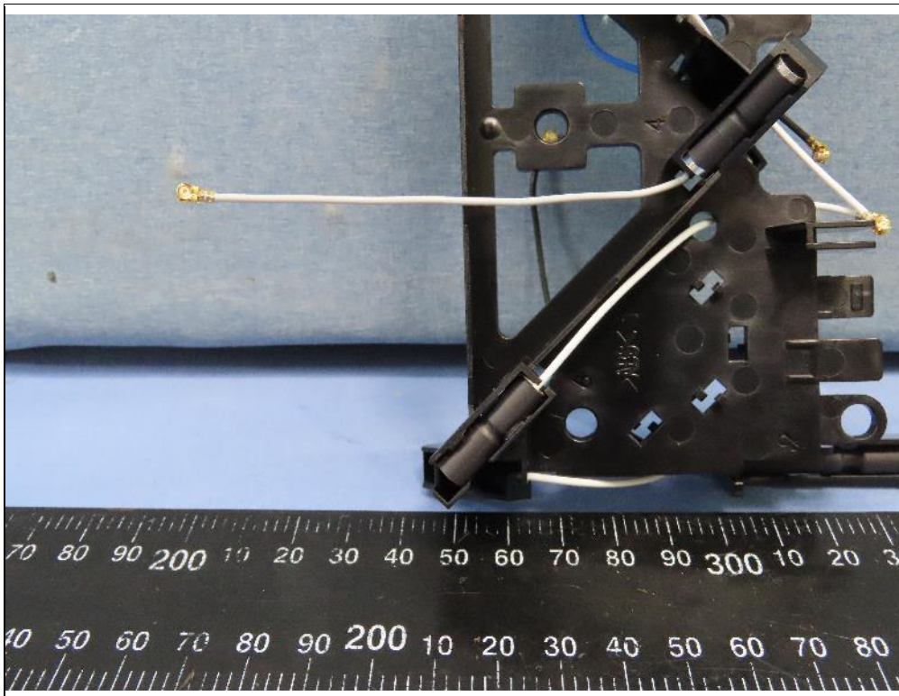
ANT_5G 3
