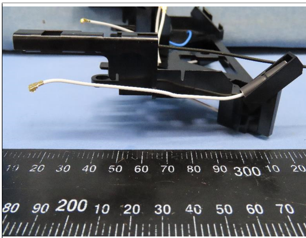
ANT_6G 2
