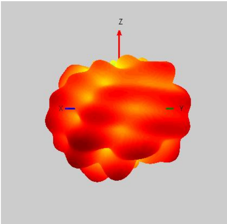
Gain&Efficiency
