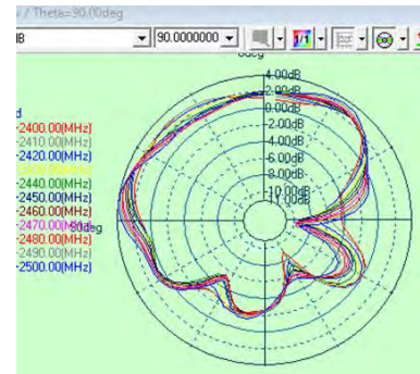
H (Theta=90)
