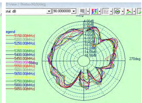
H (Theta=90)
