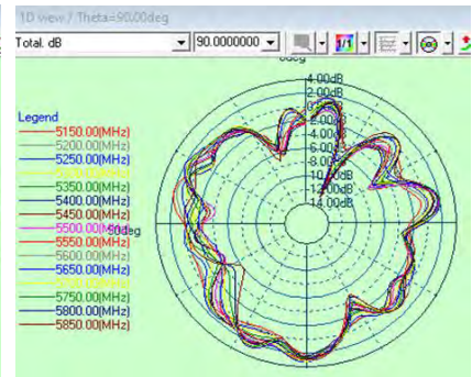
H (Theta=90)
