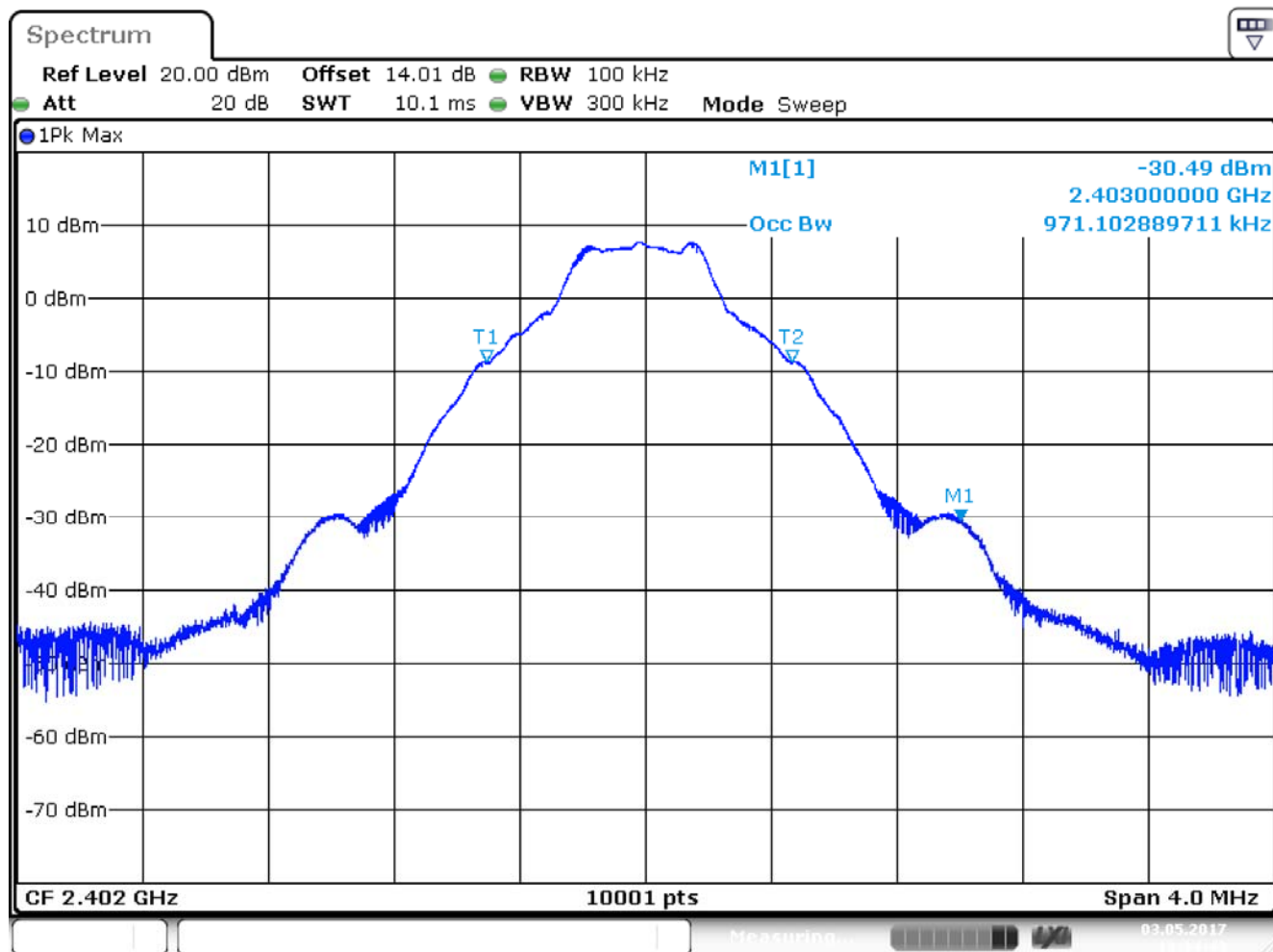
Channel 00
