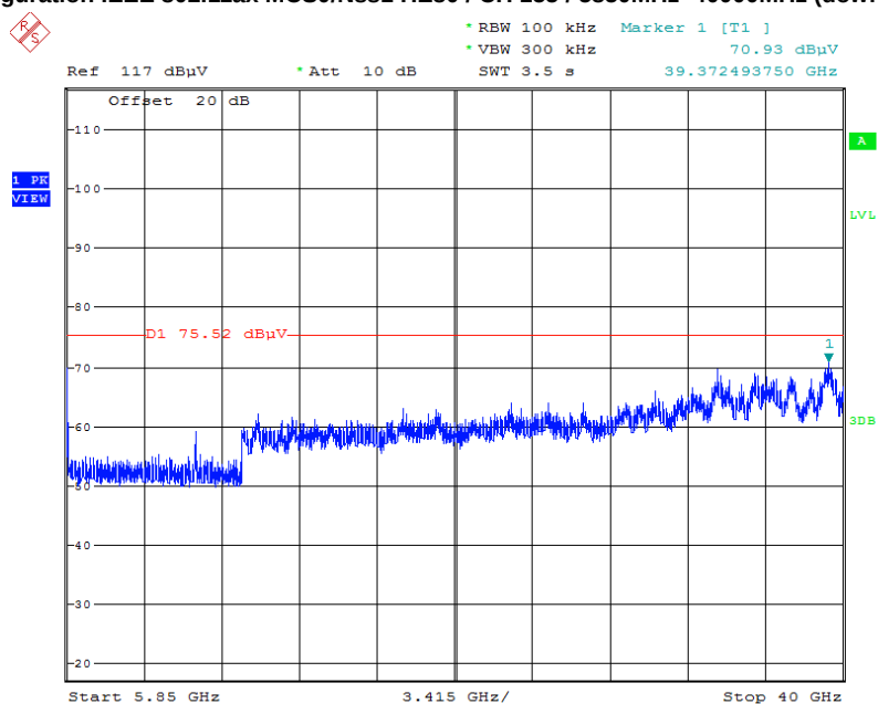
Plot on Configuration IEEE 802.11ax MCS0/Nss1 HE80 / CH 155 / 5850MHz~40000MHz (down 30dBc)
