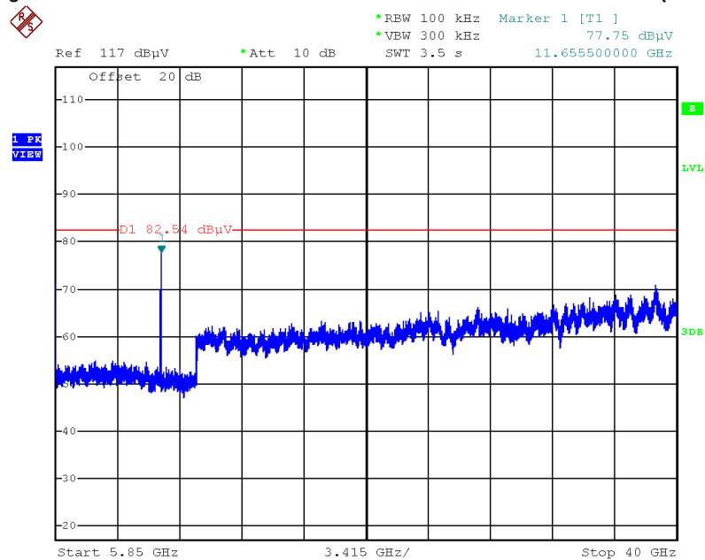
Plot on Configuration IEEE 802.11ax MCS0/Nss2 HE20 / CH 165 / 5850MHz~40000MHz (down 30dBc)
