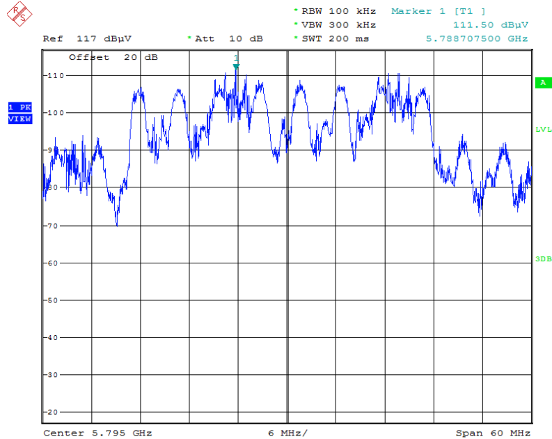
Plot on Configuration IEEE 802.11ax MCS0/Nss1 HE40 / Reference Level
