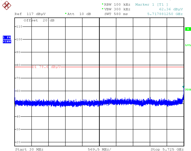
Plot on Configuration IEEE 802.11ax MCS0/Nss1 HE40 / CH 159 / 30MHz~5725MHz (down 30dBc)
