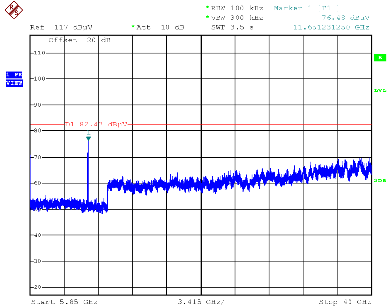
Plot on Configuration IEEE 802.11ax MCS0/Nss1 HE20 / CH 165 / 5850MHz~40000MHz (down 30dBc)
