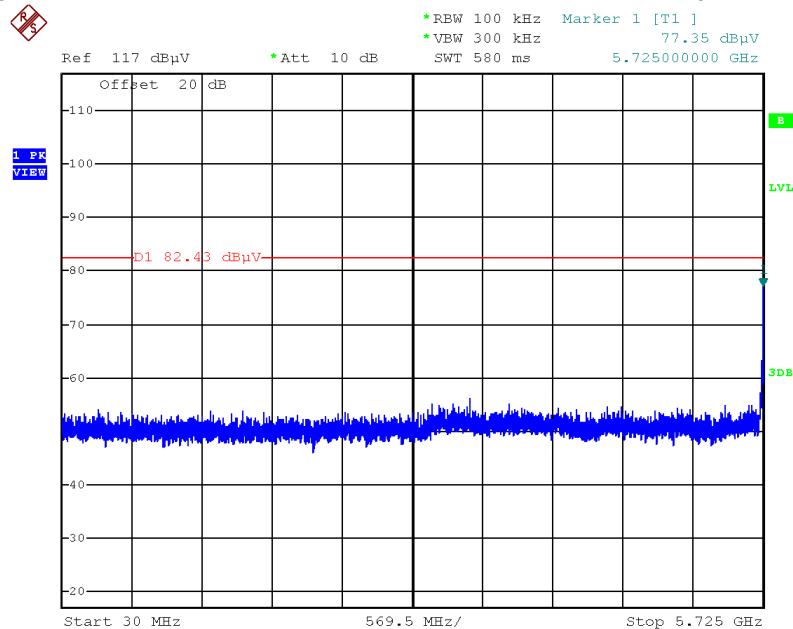
Plot on Configuration IEEE 802.11ax MCS0/Nss1 HE20 / CH 149 / 30MHz~5725MHz (down 30dBc)
