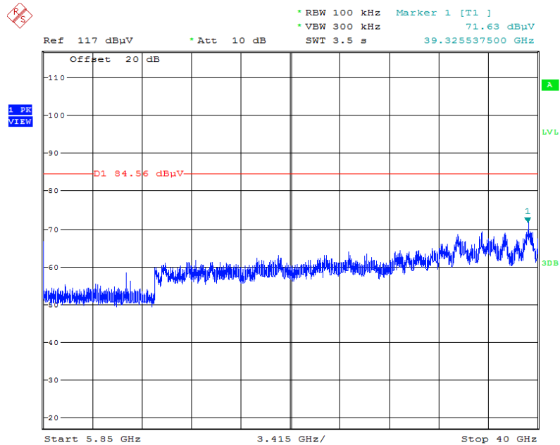
Plot on Configuration IEEE 802.11a / CH 165 / 5850MHz~40000MHz (down 30dBc)
