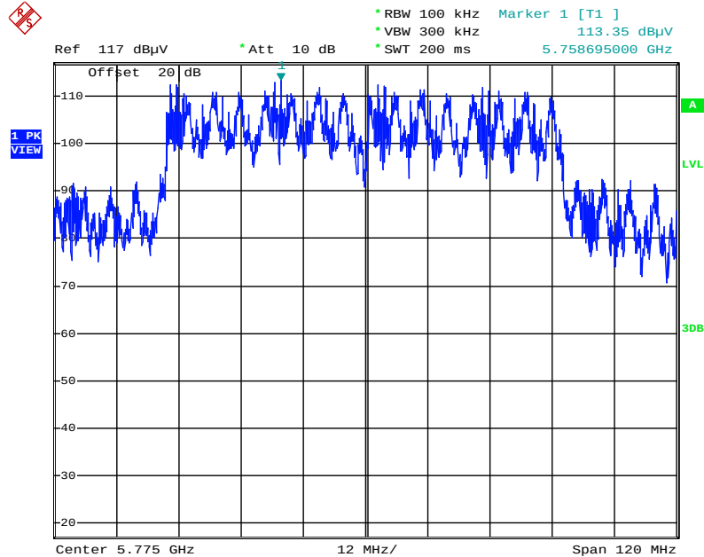
Plot on Configuration IEEE 802.11ac MCS0/Nss4 VHT 80 / Reference Level
