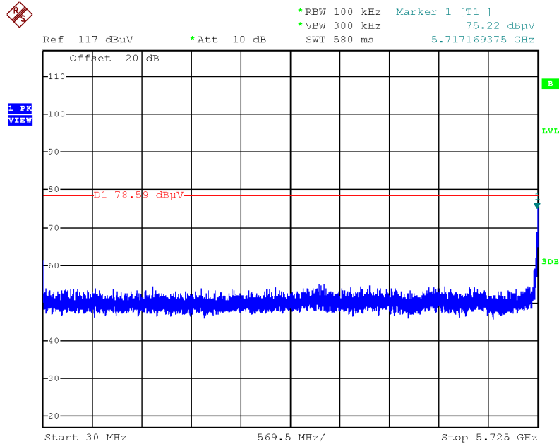
Plot on Configuration IEEE 802.11ax MCS0/Nss2 HE40 / CH 151 / 30MHz~5725MHz (down 30dBc)
