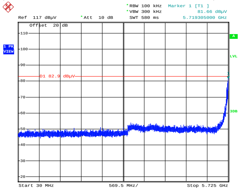
Plot on Configuration IEEE 802.11ax MCS0/Nss4 HE80 / CH 155 / 30MHz~5725MHz (down 30dBc)
