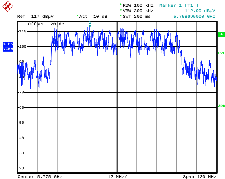
Plot on Configuration IEEE 802.11ax MCS0/Nss4 HE80 / Reference Level
