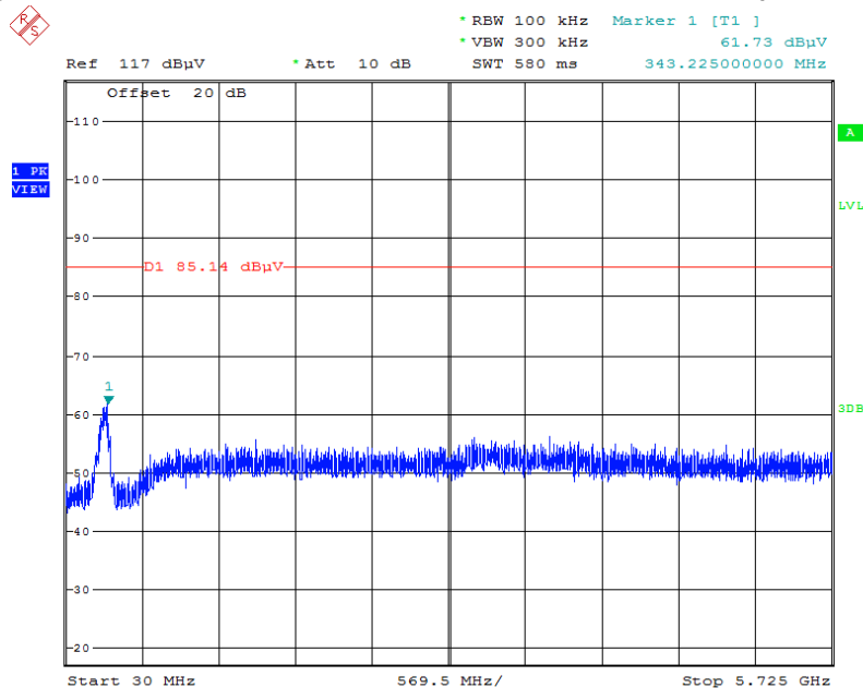
Plot on Configuration IEEE 802.11ax MCS0/Nss1 HE20 / CH 165 / 30MHz~5725MHz (down 30dBc)
