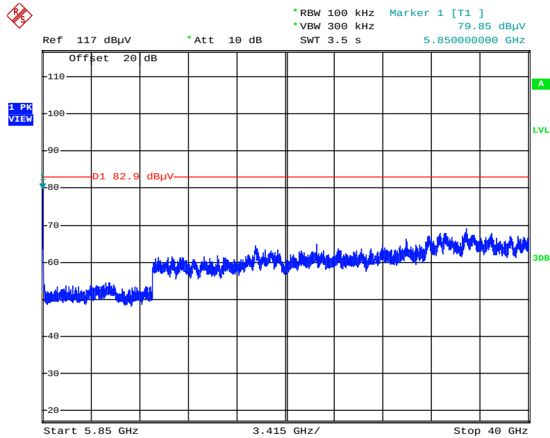
Plot on Configuration IEEE 802.11ax MCS0/Nss4 HE80 / CH 155 / 5850MHz~40000MHz (down 30dBc)
