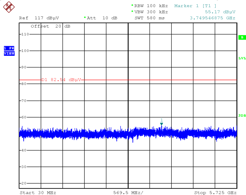
Plot on Configuration IEEE 802.11ax MCS0/Nss2 HE20 / CH 165 / 30MHz~5725MHz (down 30dBc)
