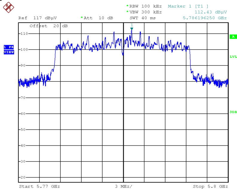
Plot on Configuration IEEE 802.11ax MCS0/Nss1 HE20 / Reference Level
