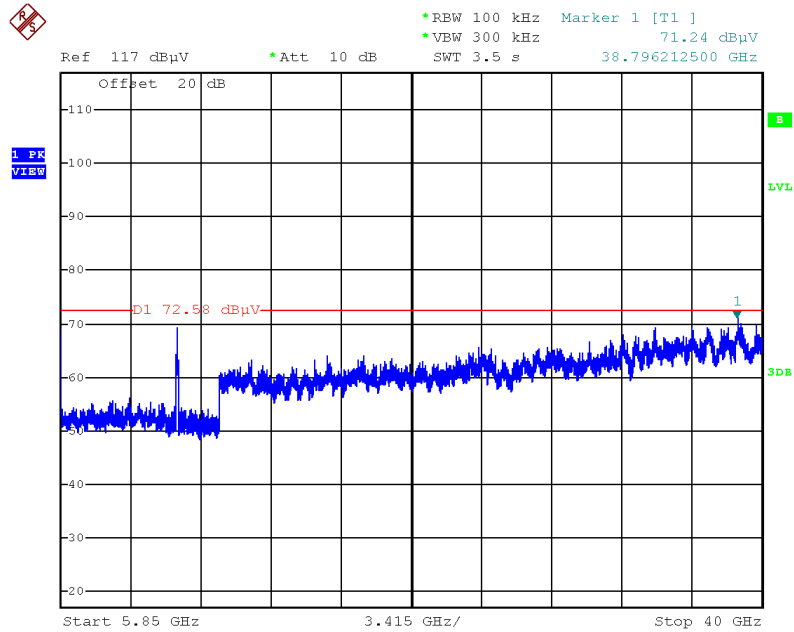
Plot on Configuration IEEE 802.11ax MCS0/Nss1 HE80 / CH 155 / 5850MHz~40000MHz (down 30dBc)
