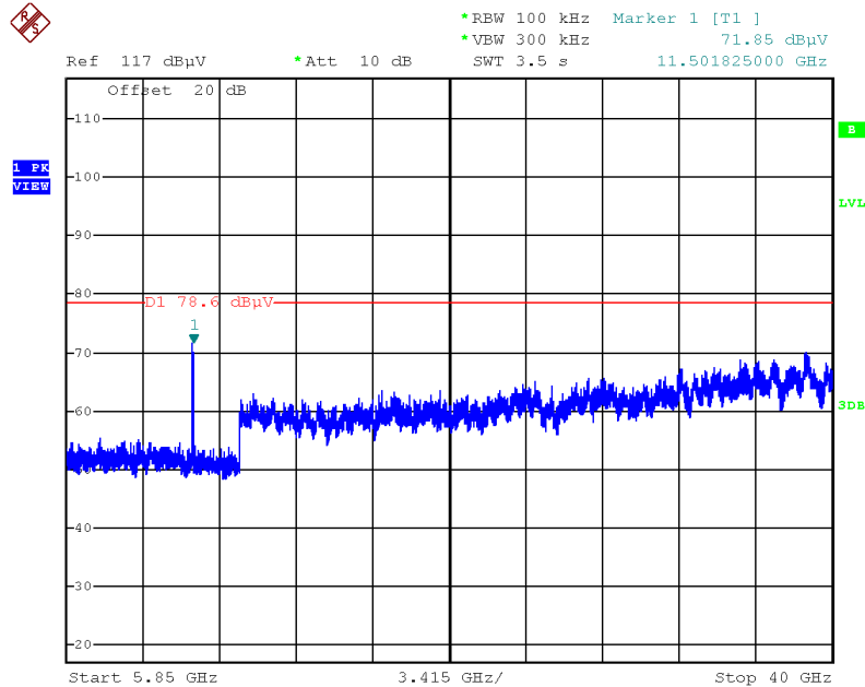
Plot on Configuration IEEE 802.11ax MCS0/Nss1 HE40 / CH 151 / 5850MHz~40000MHz (down 30dBc)
