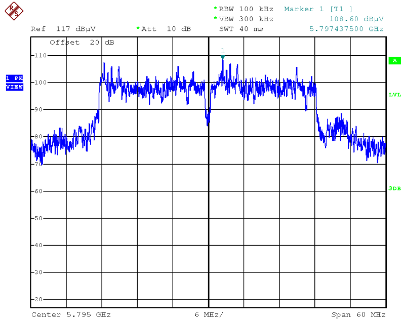
Plot on Configuration IEEE 802.11ac MCS0/Nss2 VHT40 / Reference Level
