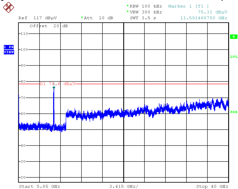
Plot on Configuration IEEE 802.11ax MCS0/Nss1 HE40 / CH 159 / 5850MHz~40000MHz (down 30dBc)
