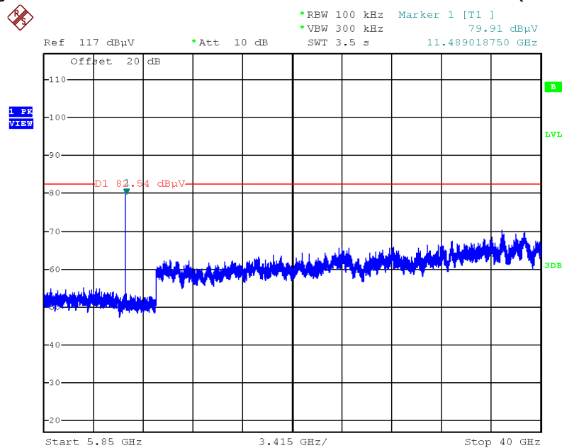
Plot on Configuration IEEE 802.11ax MCS0/Nss2 HE20 / CH 149 / 5850MHz~40000MHz (down 30dBc)
