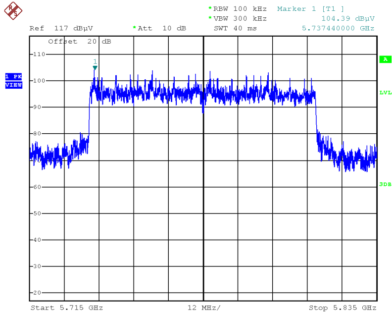
Plot on Configuration IEEE 802.11ax MCS0/Nss2 HE80 / Reference Level
