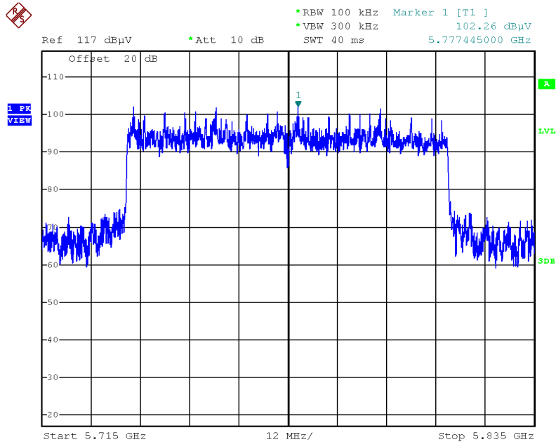
Plot on Configuration IEEE 802.11ac MCS0/Nss1 VHT80 / Reference Level
