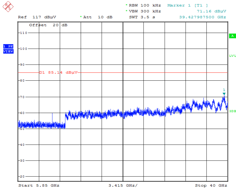
Plot on Configuration IEEE 802.11ax MCS0/Nss1 HE20 / CH 149 / 5850MHz~40000MHz (down 30dBc)
