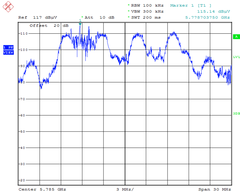
Plot on Configuration IEEE 802.11ax MCS0/Nss1 HE20 / Reference Level
