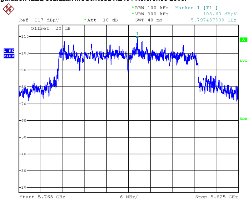
Plot on Configuration IEEE 802.11ax MCS0/Nss1 HE40 / Reference Level
