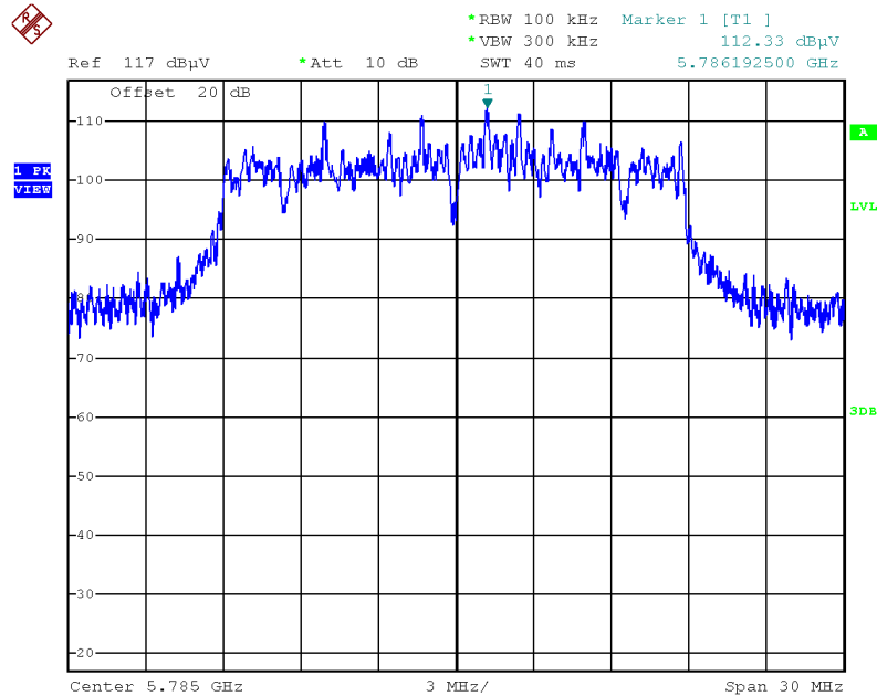
Plot on Configuration IEEE 802.11ac MCS0/Nss2 VHT20 / Reference Level
