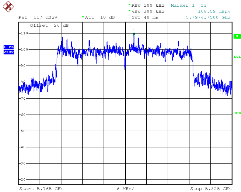
Plot on Configuration IEEE 802.11ax MCS0/Nss2 HE40 / Reference Level
