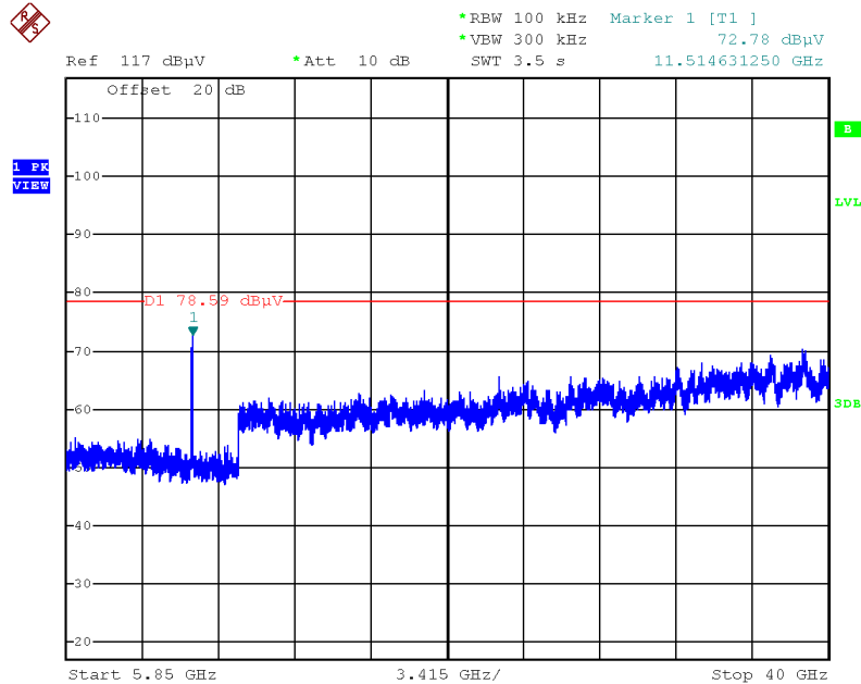
Plot on Configuration IEEE 802.11ax MCS0/Nss2 HE40 / CH 151 / 5850MHz~40000MHz (down 30dBc)
