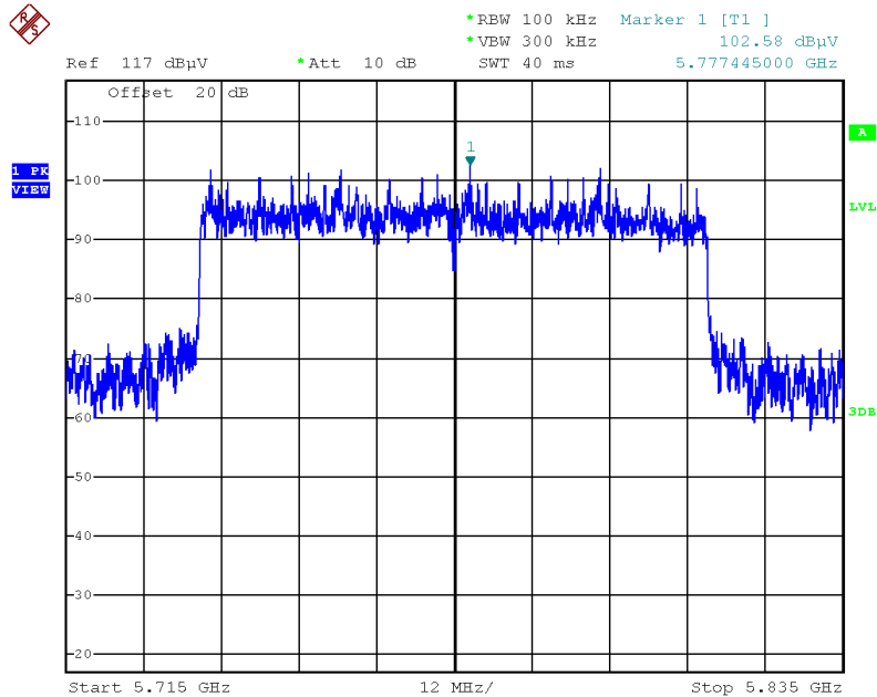
Plot on Configuration IEEE 802.11ax MCS0/Nss1 HE80 / Reference Level
