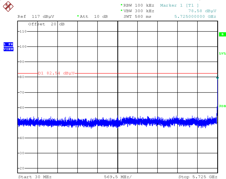
Plot on Configuration IEEE 802.11ax MCS0/Nss2 HE20 / CH 149 / 30MHz~5725MHz (down 30dBc)
