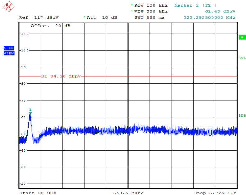
Plot on Configuration IEEE 802.11a / CH 165 / 30MHz~5725MHz (down 30dBc)
