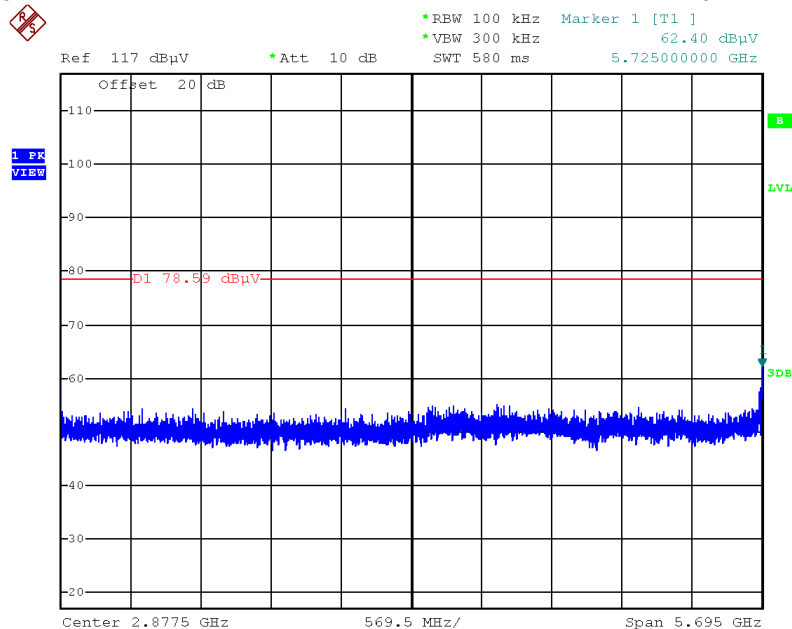
Plot on Configuration IEEE 802.11ax MCS0/Nss2 HE40 / CH 159 / 30MHz~5725MHz (down 30dBc)
