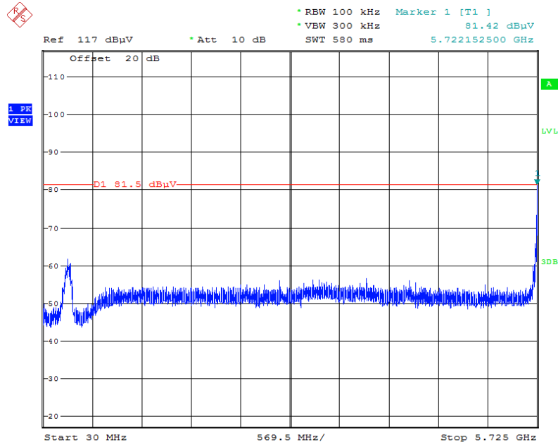
Plot on Configuration IEEE 802.11ax MCS0/Nss1 HE40 / CH 151 / 30MHz~5725MHz (down 30dBc)
