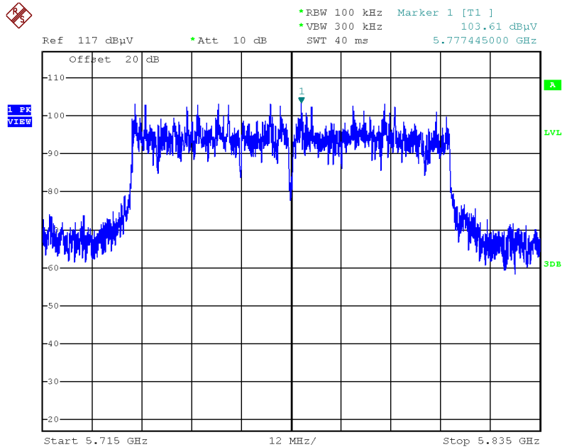
Plot on Configuration IEEE 802.11ac MCS0/Nss2 VHT80 / Reference Level
