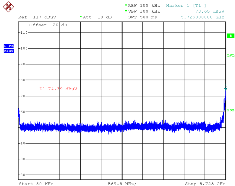
Plot on Configuration IEEE 802.11ax MCS0/Nss2 HE80 / CH 155 / 30MHz~5725MHz (down 30dBc)
