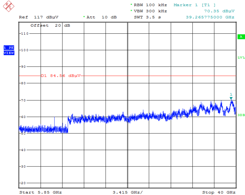
Plot on Configuration IEEE 802.11a / CH 149 / 5850MHz~40000MHz (down 30dBc)
