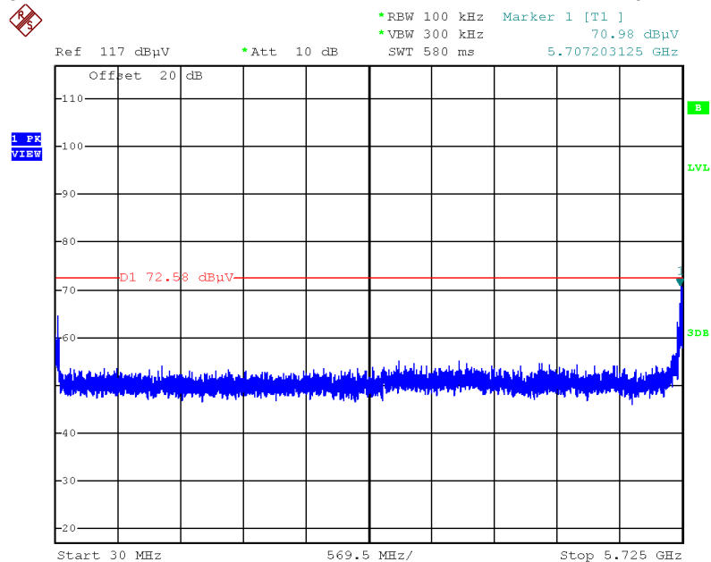
Plot on Configuration IEEE 802.11ax MCS0/Nss1 HE80 / CH 155 / 30MHz~5725MHz (down 30dBc)
