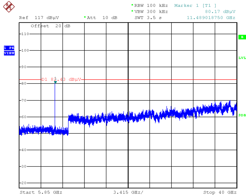
Plot on Configuration IEEE 802.11ax MCS0/Nss1 HE20 / CH 149 / 5850MHz~40000MHz (down 30dBc)
