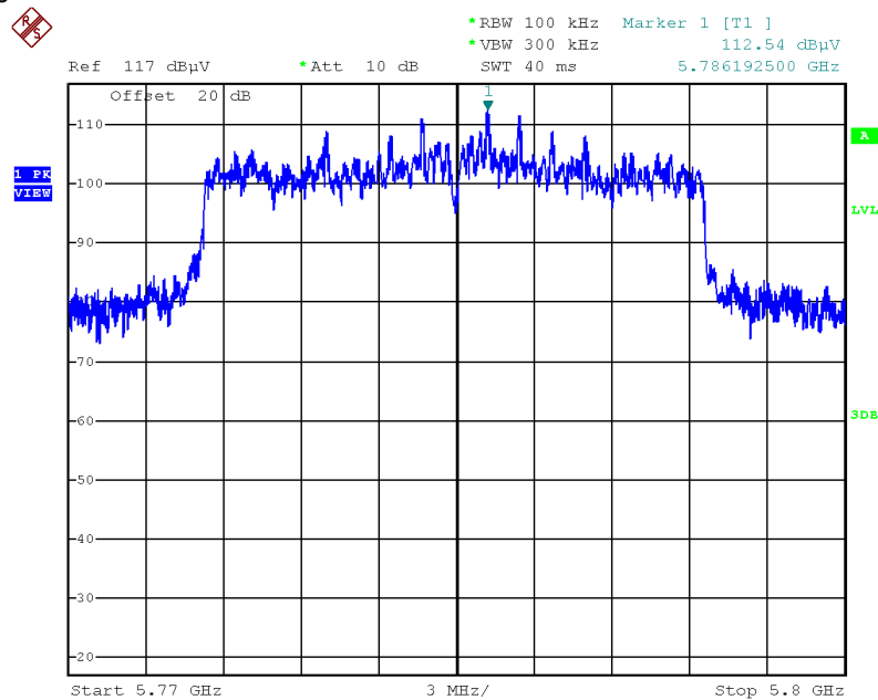
Plot on Configuration IEEE 802.11ax MCS0/Nss2 HE20 / Reference Level
