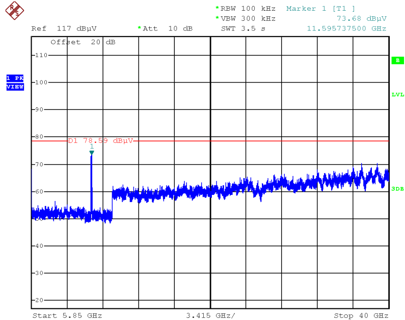
Plot on Configuration IEEE 802.11ax MCS0/Nss2 HE40 / CH 159 / 5850MHz~40000MHz (down 30dBc)
