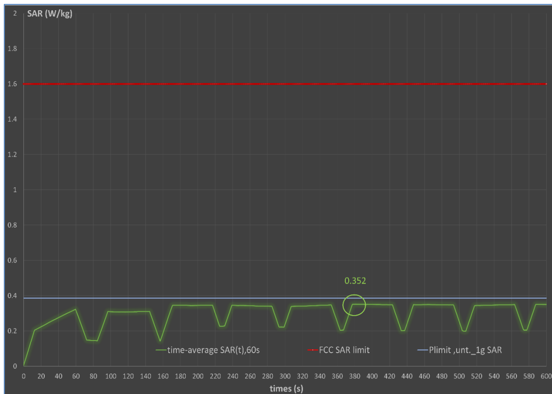
Figure 7-2: Time-Averaged SAR Measurement Result for Test Scenario 3
