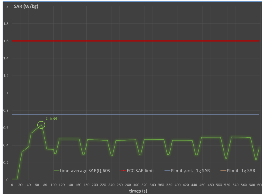
Figure 6-3: Time-Averaged SAR Over Time for Test Scenario 1
