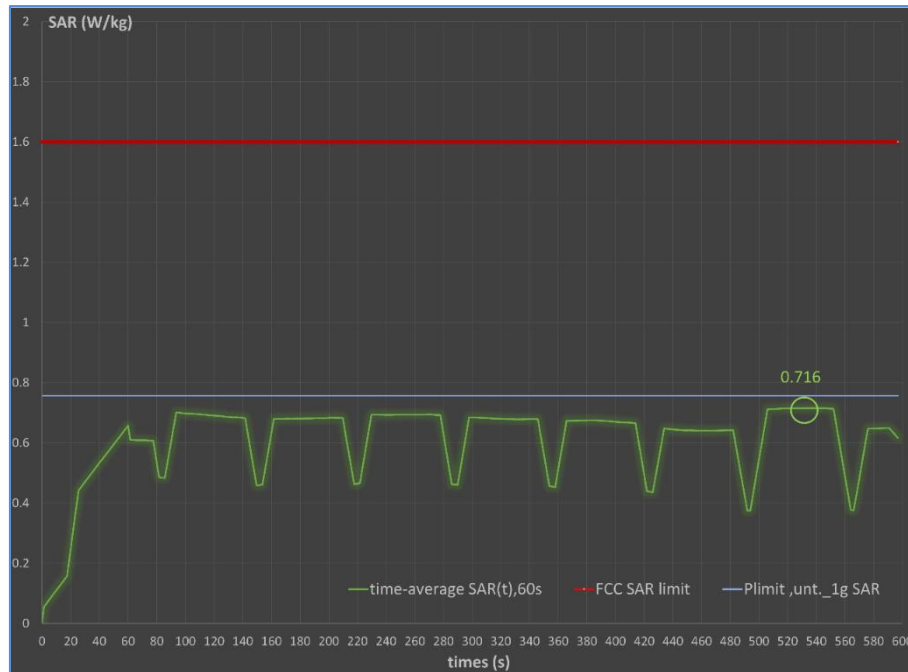
Figure 7-2: Time-Averaged SAR Measurement Result for Test Scenario 3
