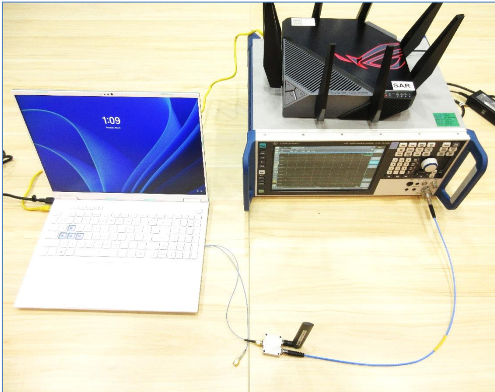
Setup for Conducted Power Testing (Test Scenario 1)
