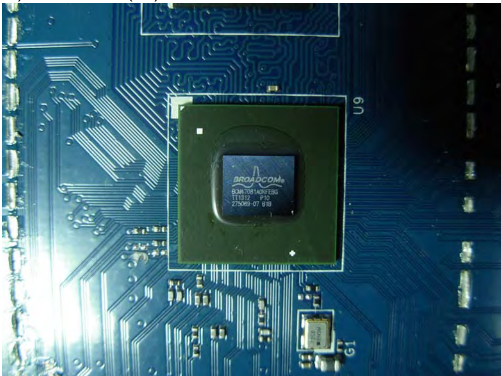
(134) EUT Photo (MB)
