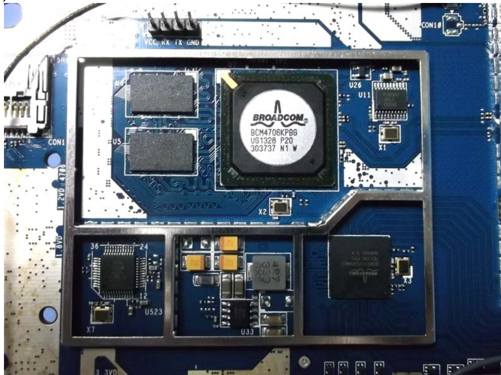
(32) EUT Photo
