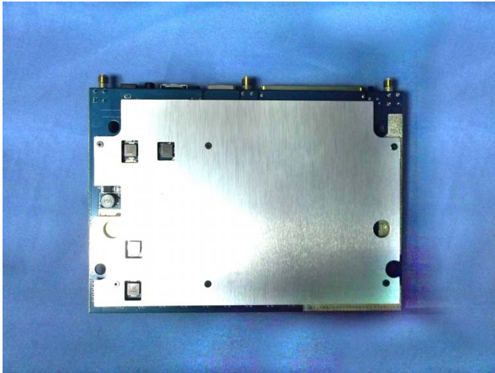
(25) EUT Photo
