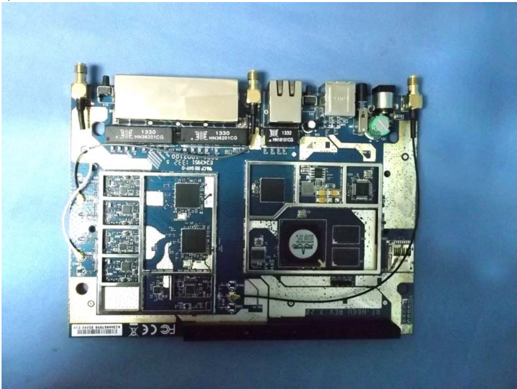
(30)EUT Photo
