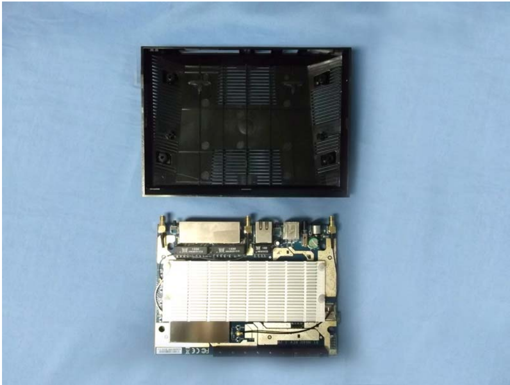
(23)EUT Photo
