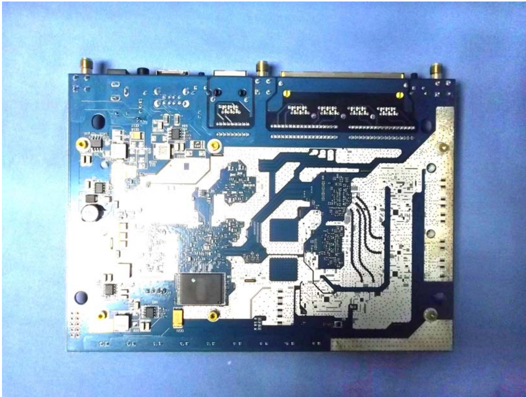
(28) EUT Photo
