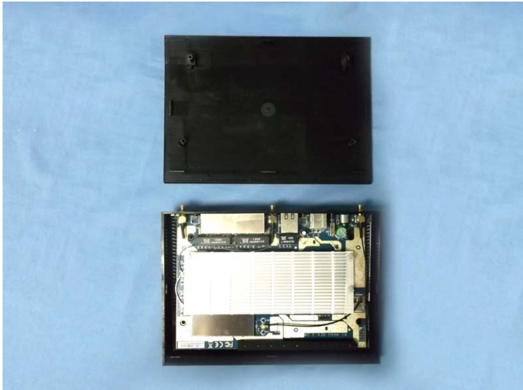
(21)EUT Photo
