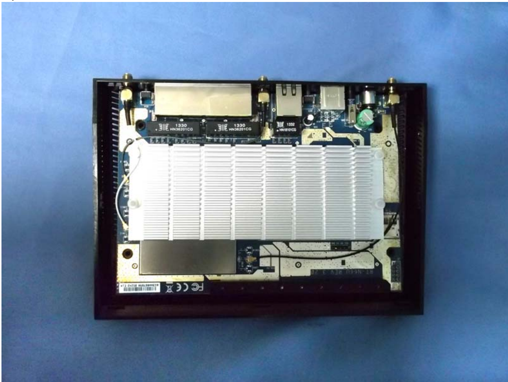
(22)EUT Photo
