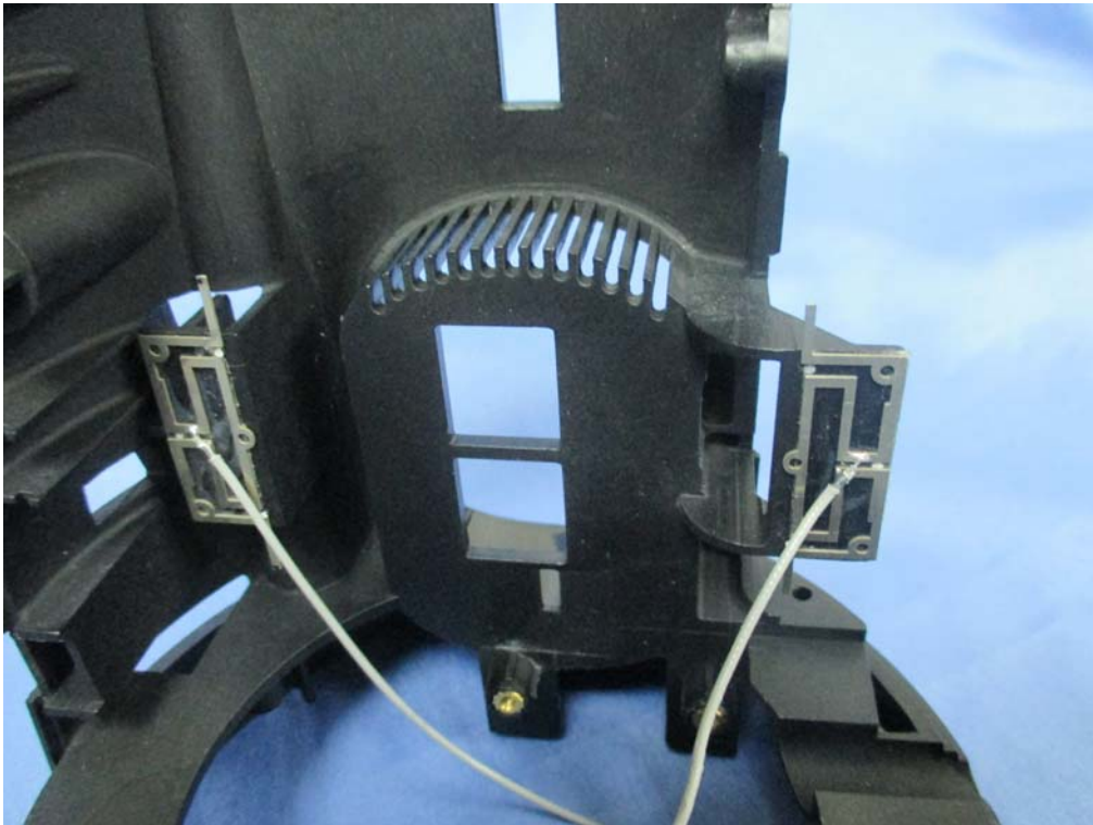
(47) EUT Photo (BT & Zigbee)
