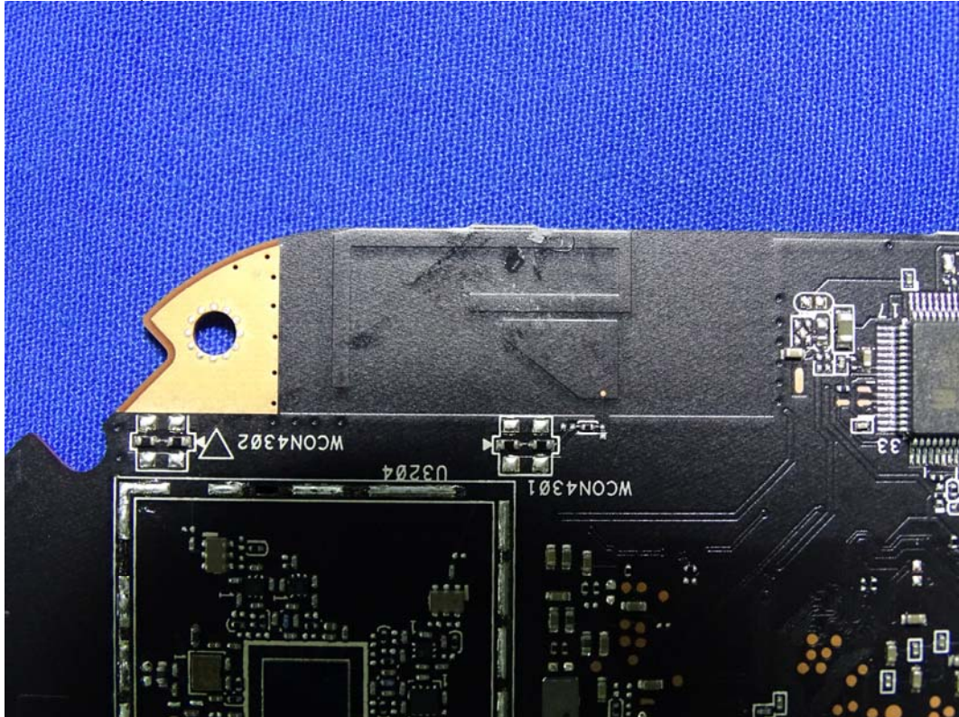
(10) EUT Photo (WiFi Antenna)
