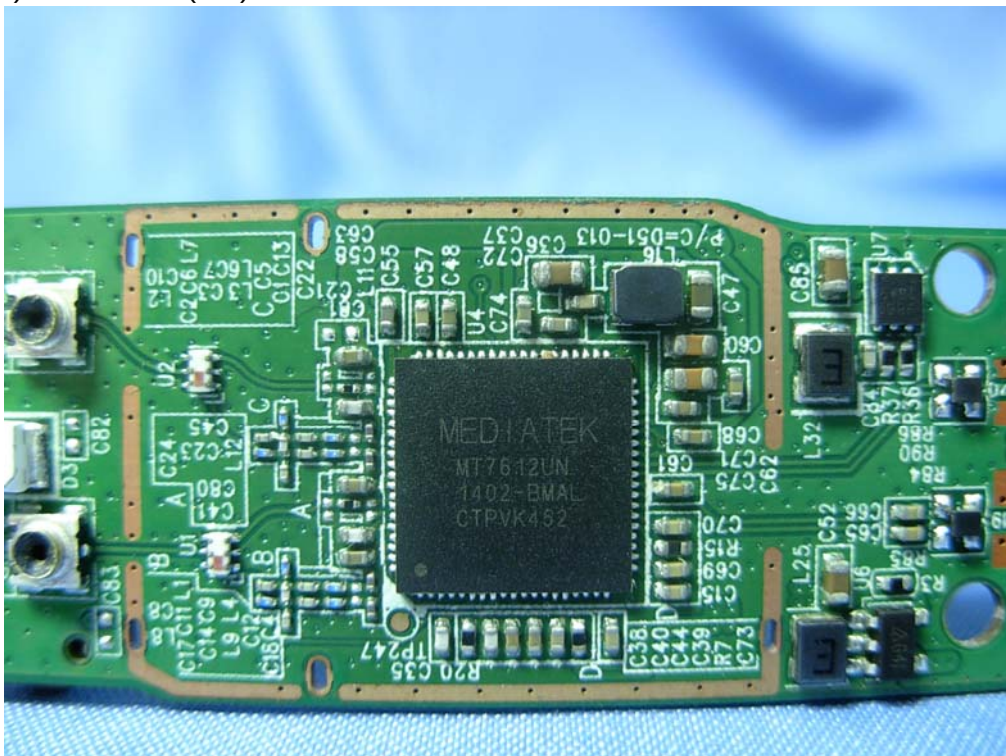
(11) EUT Photo (MB)
