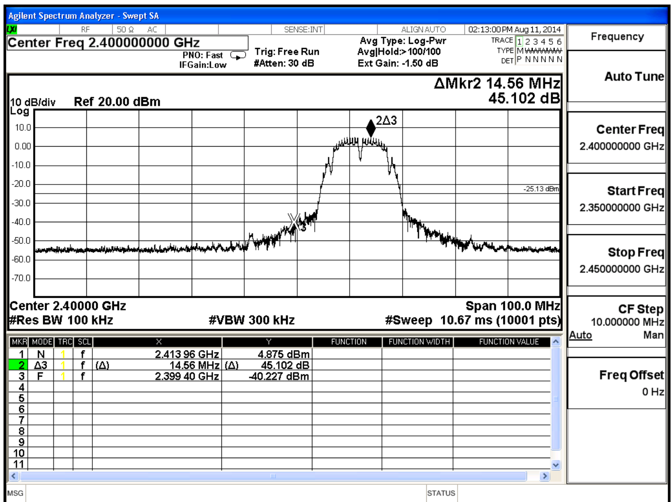
Channel 01 (2412MHz)
