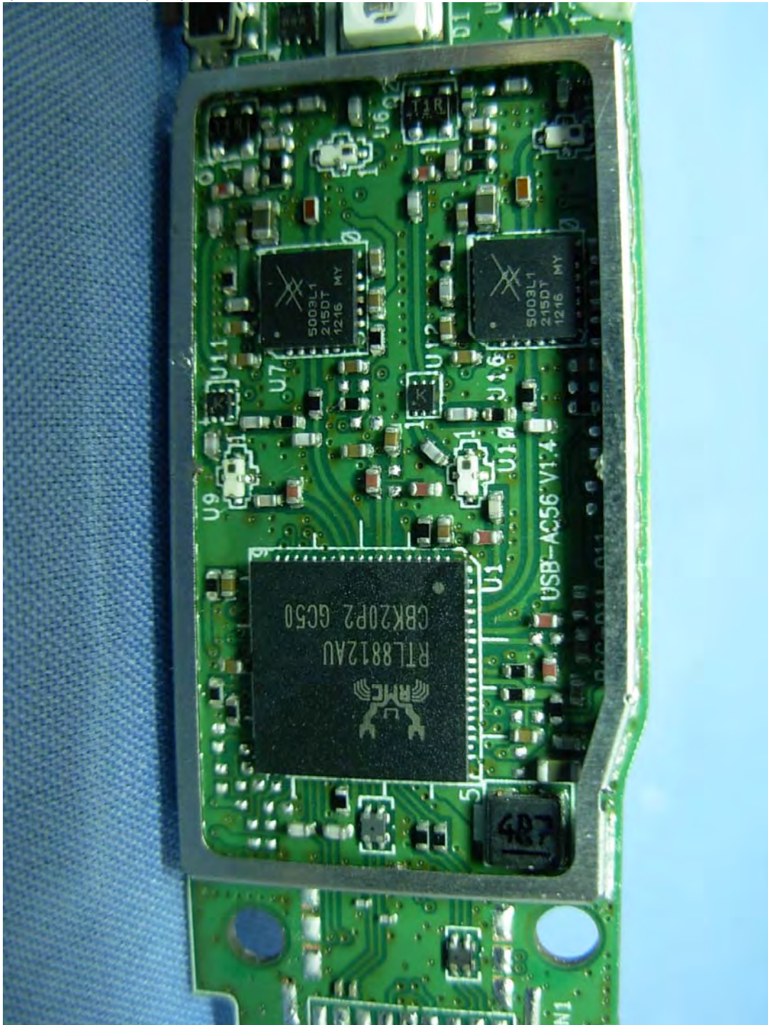
(7) EUT Photo (MB)
