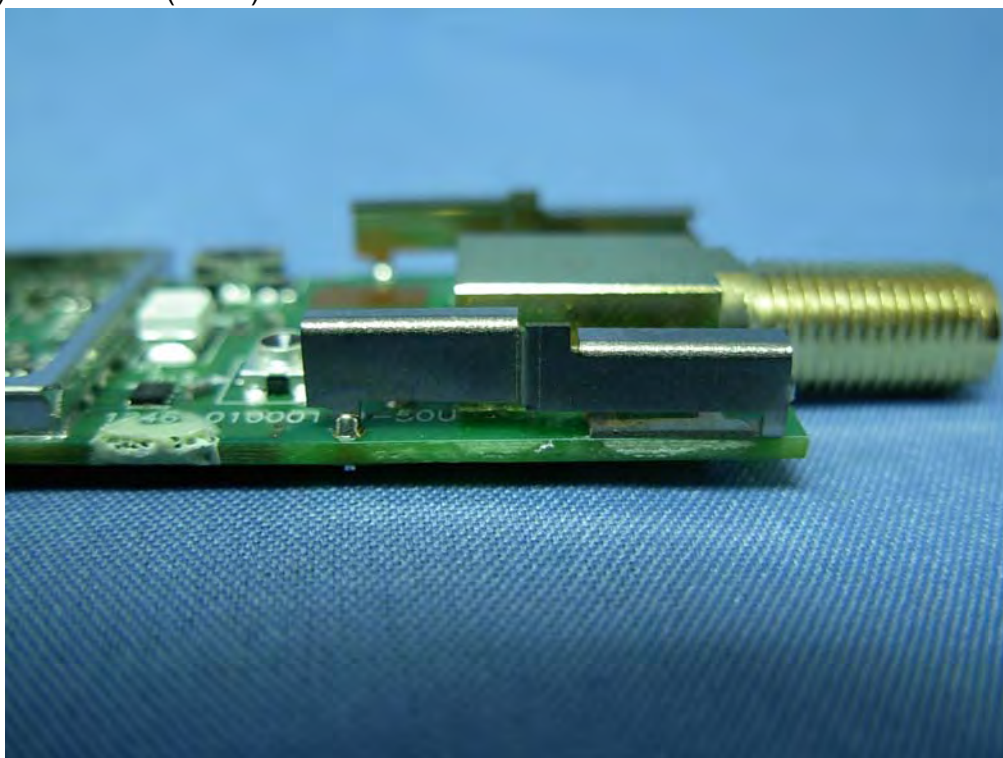
(13) EUT Photo (Dipole Antenna 0)
