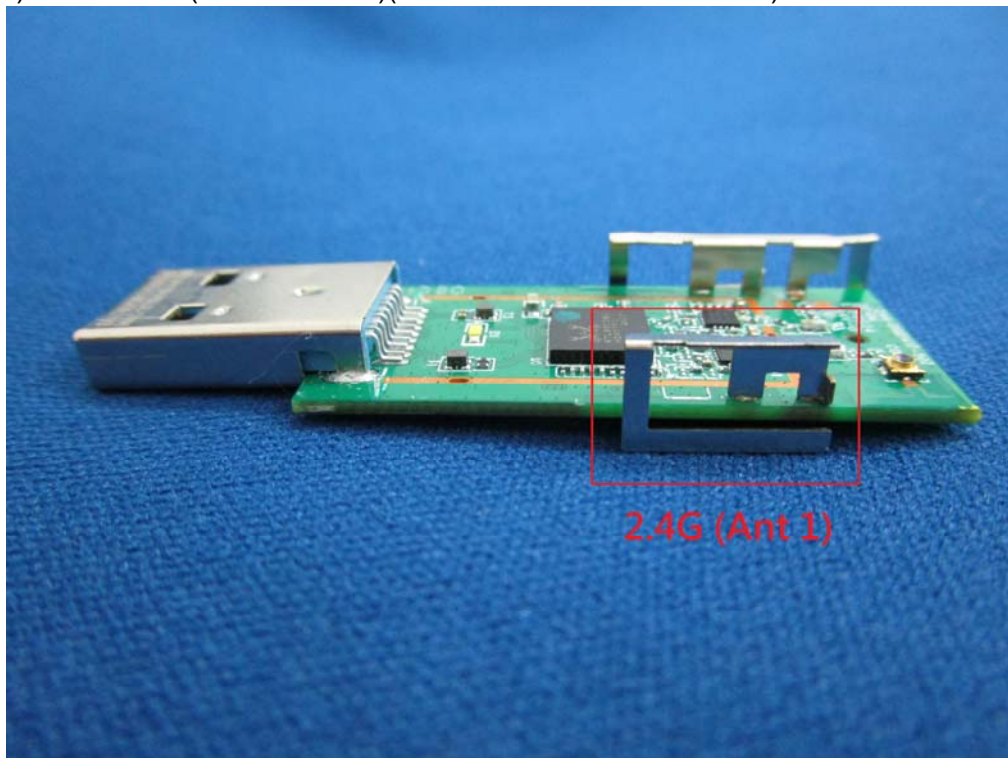
(13) EUT Photo (2.4G Antenna)(LYNwave / ALX17M-052XX1)
