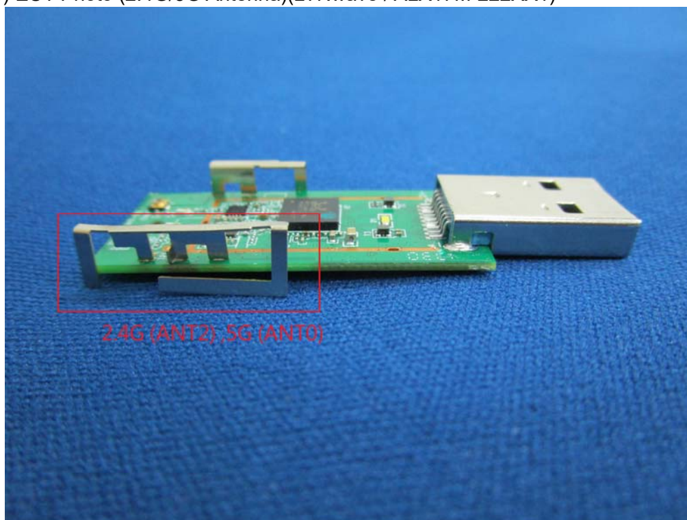
(15) EUT Photo (2.4G/5G Antenna)(LYNwave / ALX17M-222XX1)
