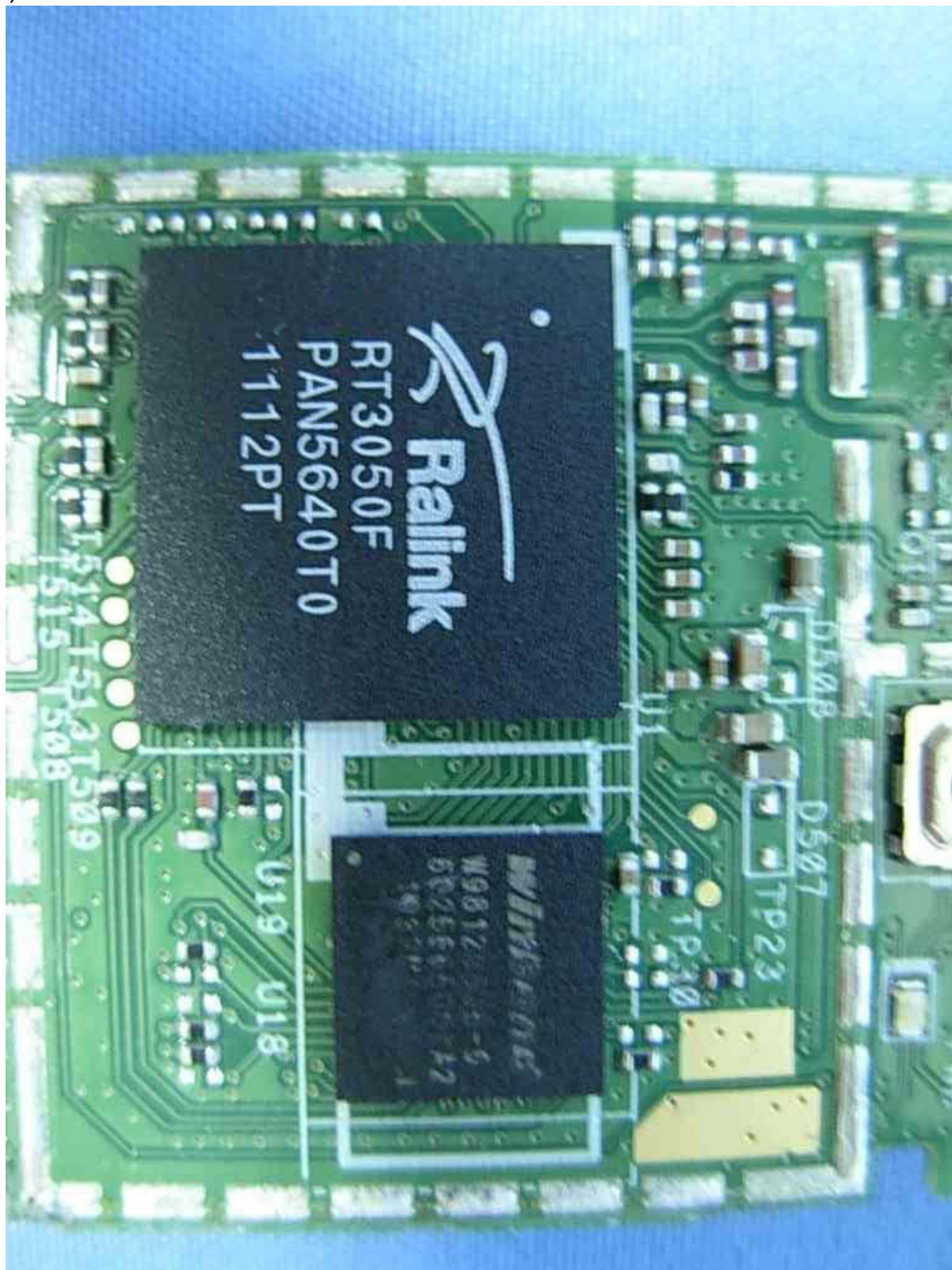
(29) EUT Photo
