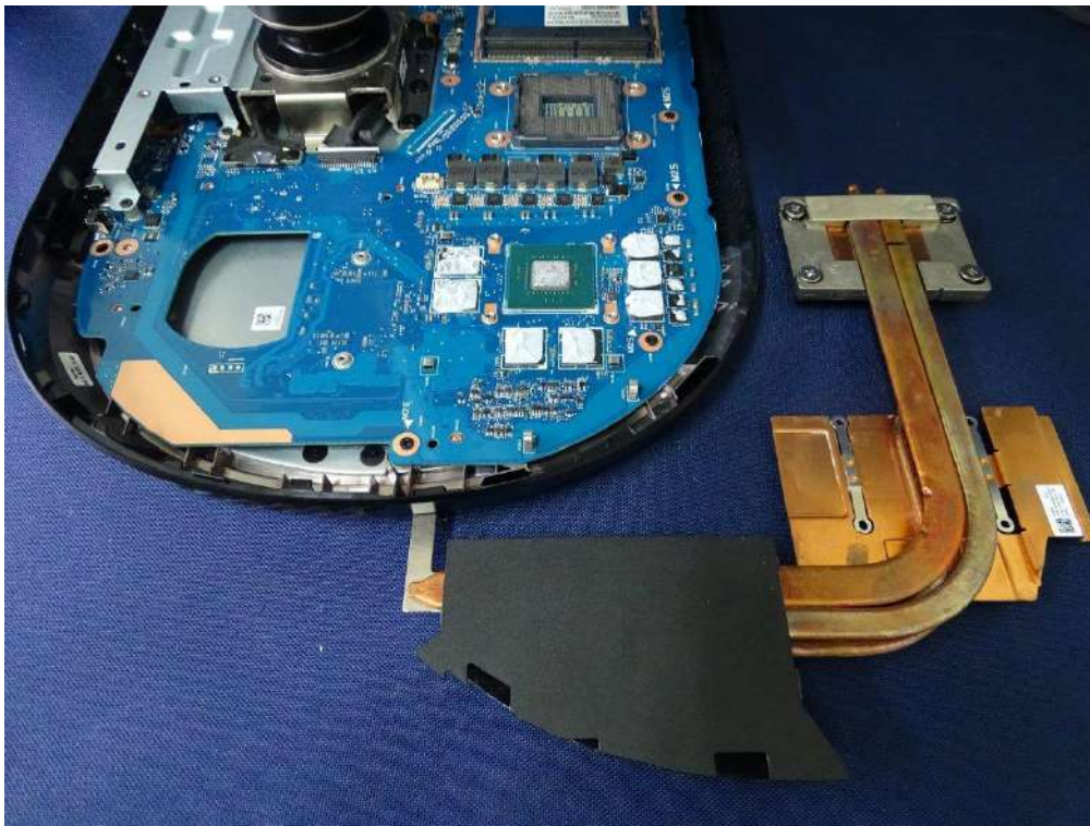
(35) EUT Photo
