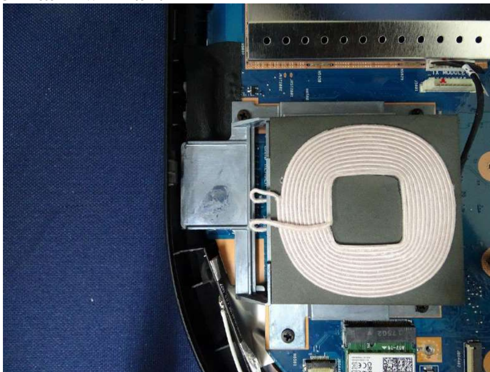
(25) EUT Photo WPT Antenna
