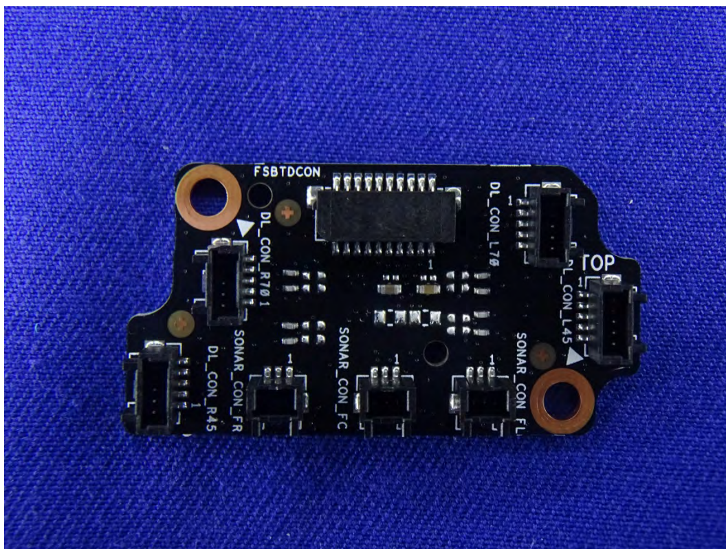
(80) EUT Photo
