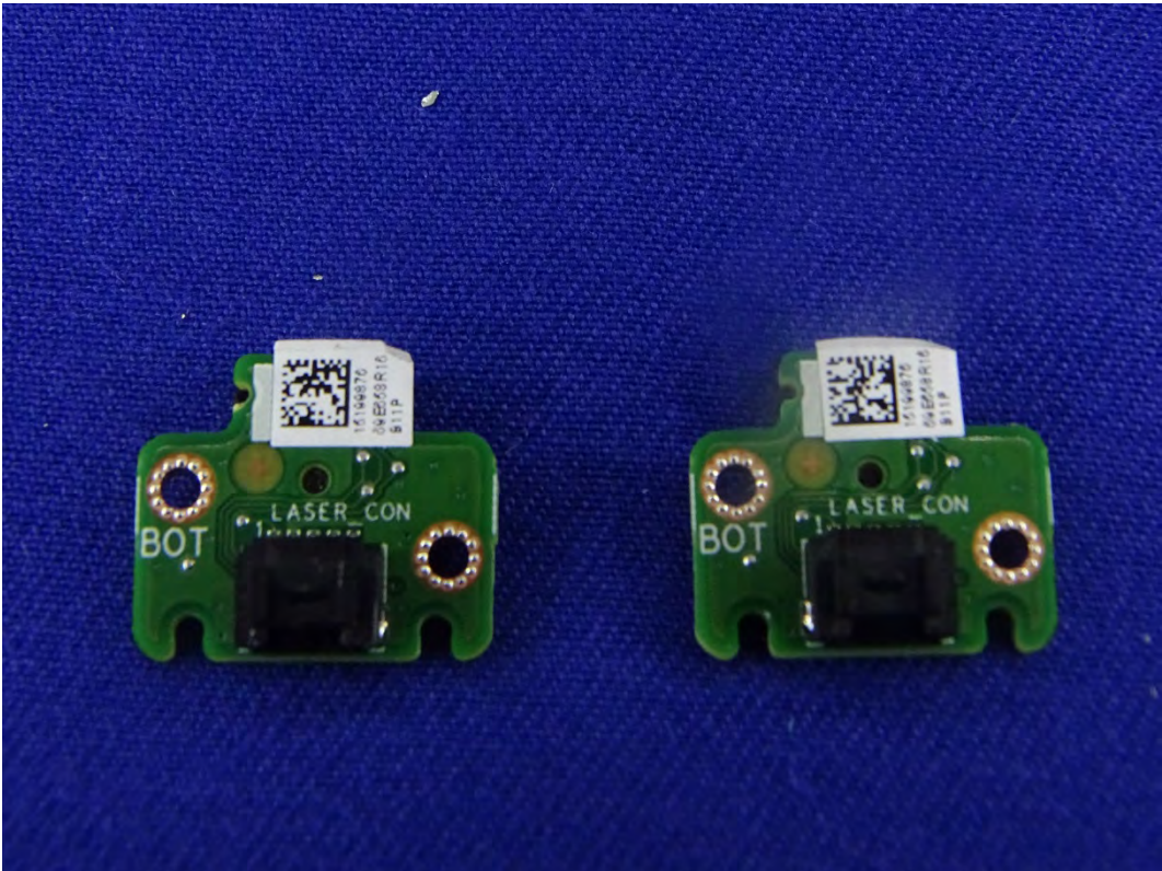
(76) EUT Photo
