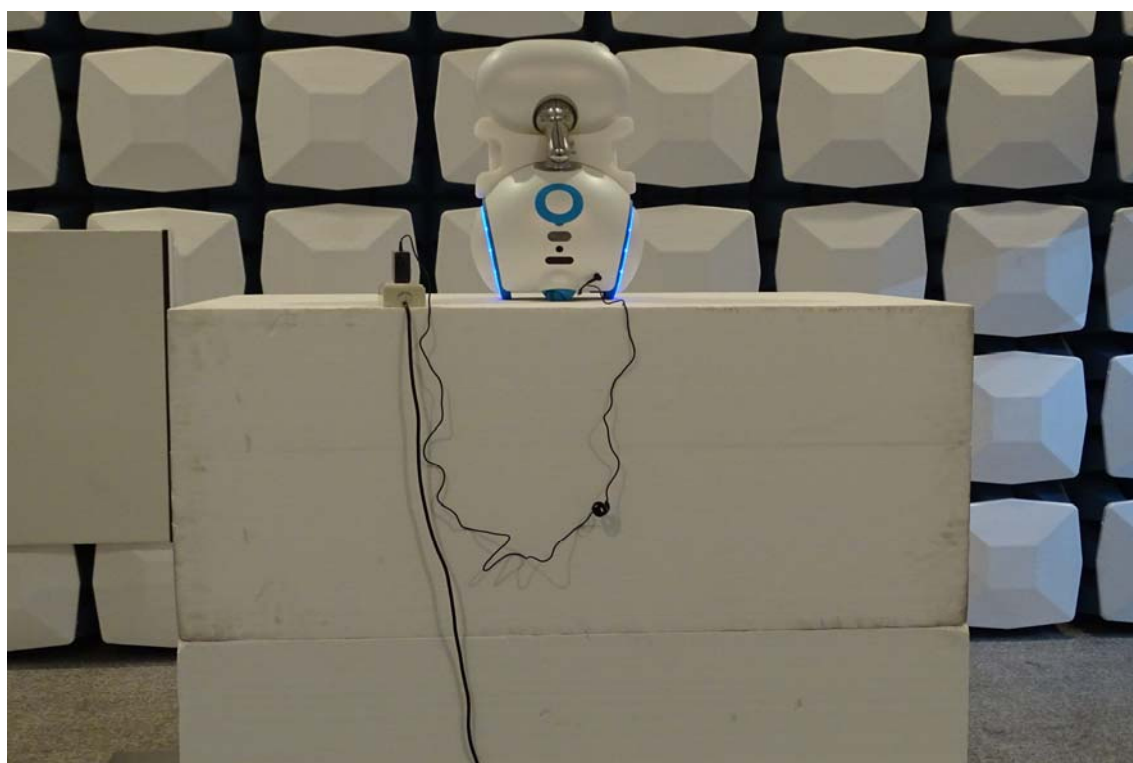
Back View of Radiated Test (Horn)
