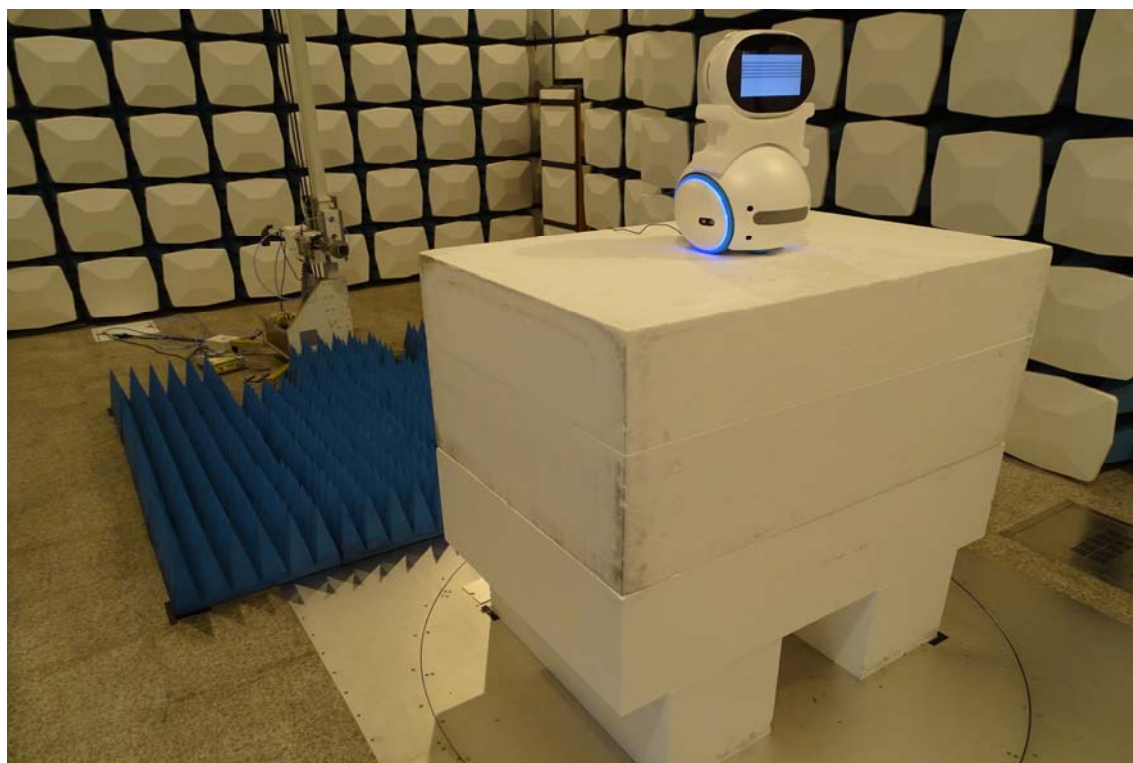
Front View of Radiated Test (Horn)
