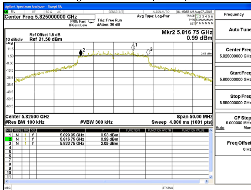
Figure Channel 165: (ChainB)
