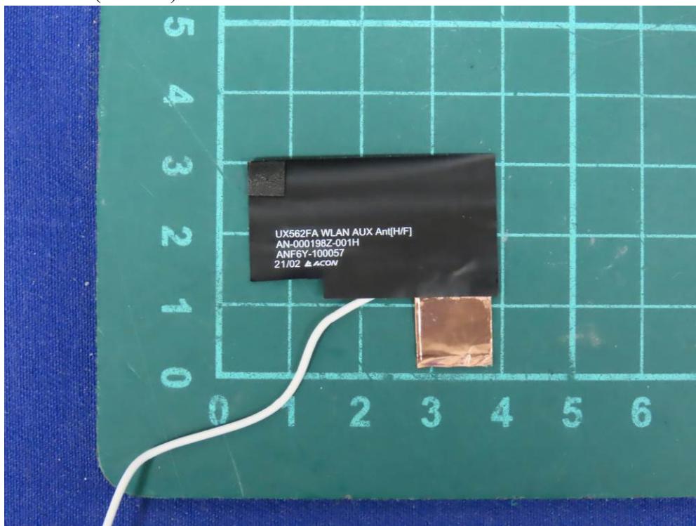
(22) EUT Photo (Antenna)
