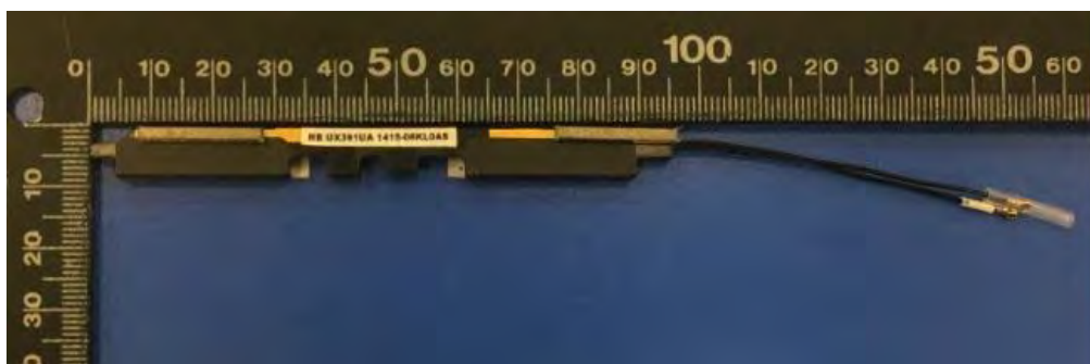
Hong Bo Main Aux Antenna Vendor 260-26213 (MAIN and Aux) ASUS 14008-03280000 (MAIN and Aux)
