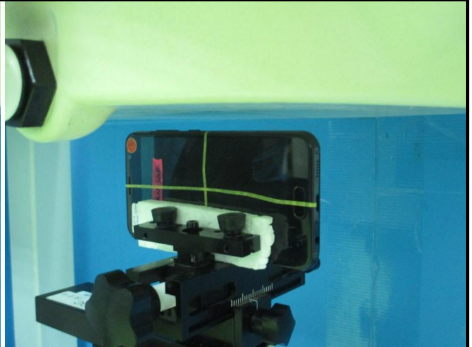
Right Side of EUT with 10 mm Gap
