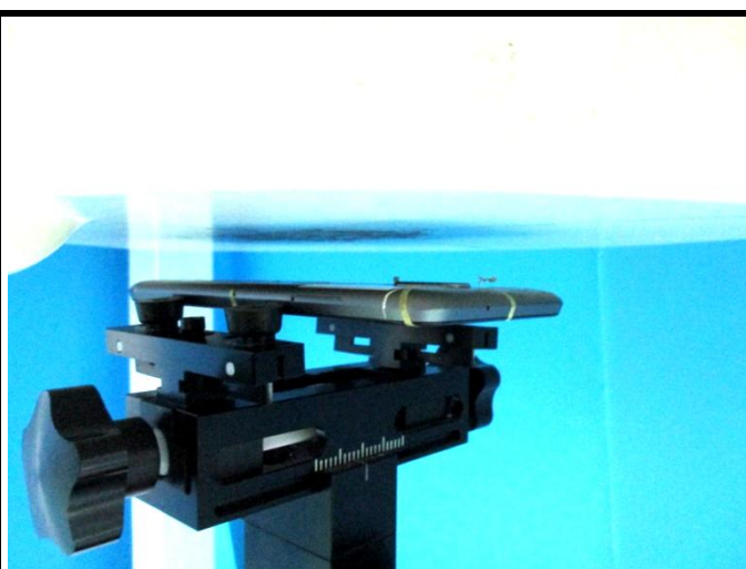
Body worn - Rear Face of EUT at 15 mm
