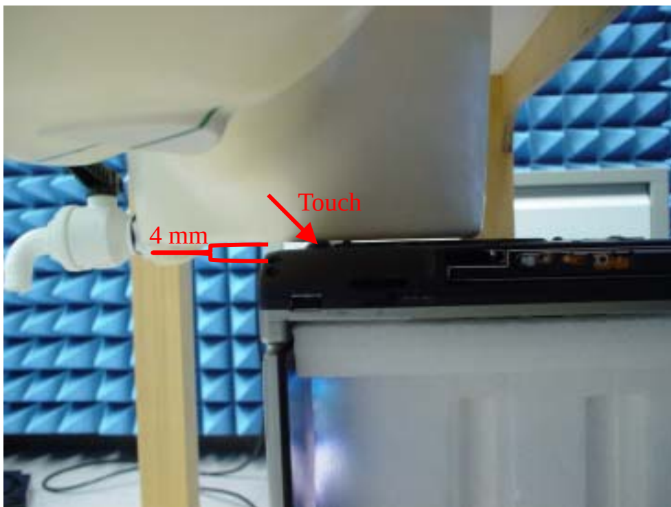
Fig.6 Photograph of the Bottom face of the EUT is paralleled with flat phantom. Spacing between EUT and phantom - In contact (0 cm)
