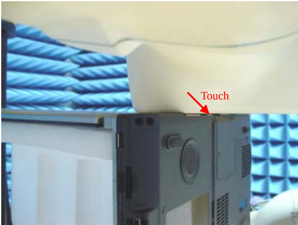
Fig.5 Photograph of the Rear side of the EUT is paralleled with flat Phantom; Spacing between EUT and phantom - In contact (0 cm).
