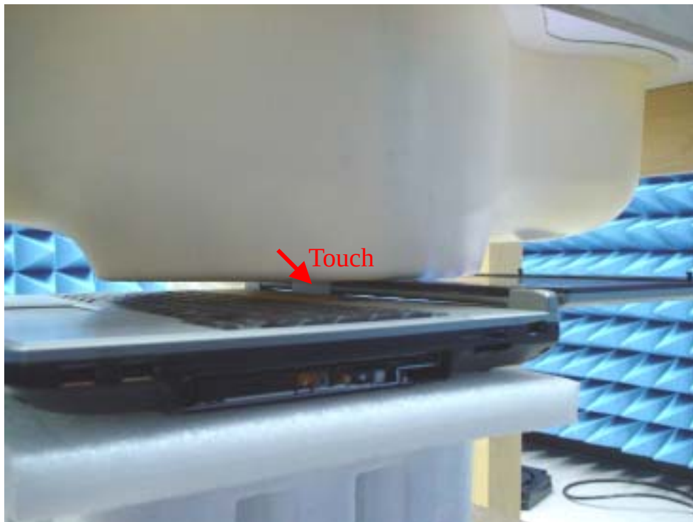
Fig.7 Photograph of the LCD panel of EUT contact to the flat phantom. The transmitting antenna of the EUT located under the reference point of the flat phantom, Spacing between EUT and phantom - In contact (0 cm)
