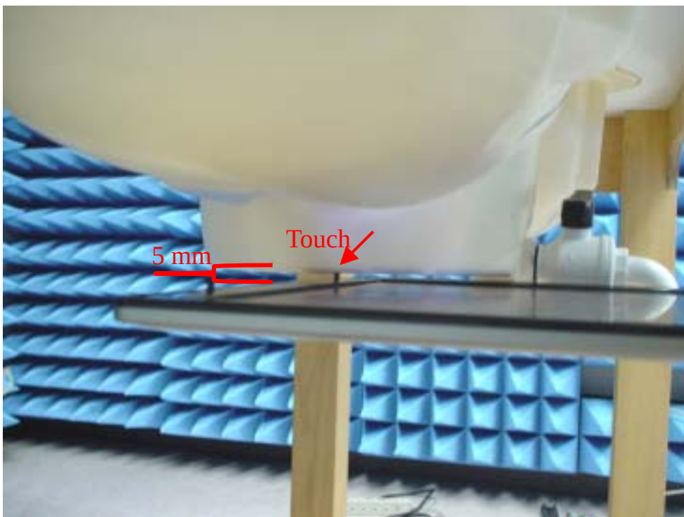
Fig.4 Photograph of the LCD panel of EUT contact to the flat phantom. Since there is a hook on the edge of panel, the panel itself can not touch phantom. Spacing between hook and phantom - In contact (0 mm)
