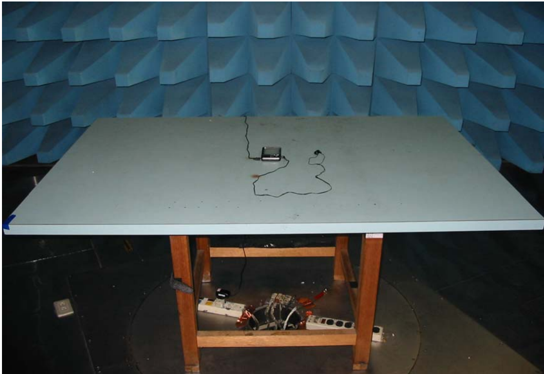
Front View of the Test Configuration of X-axis
