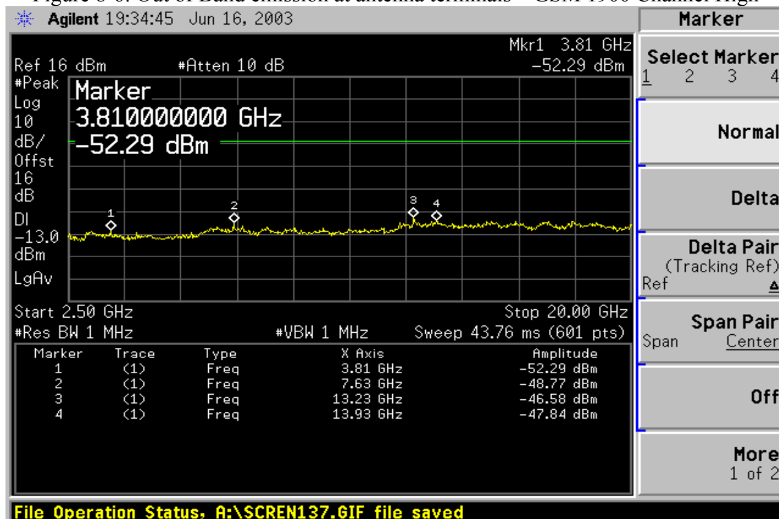
Figure 8-6: Out of Band emission at antenna terminals – GSM 1900 Channel High
