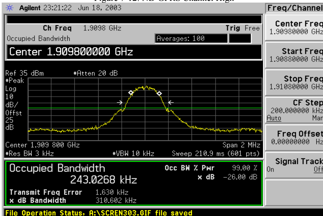
Figure 7-12: NB-GPRS Channel High
