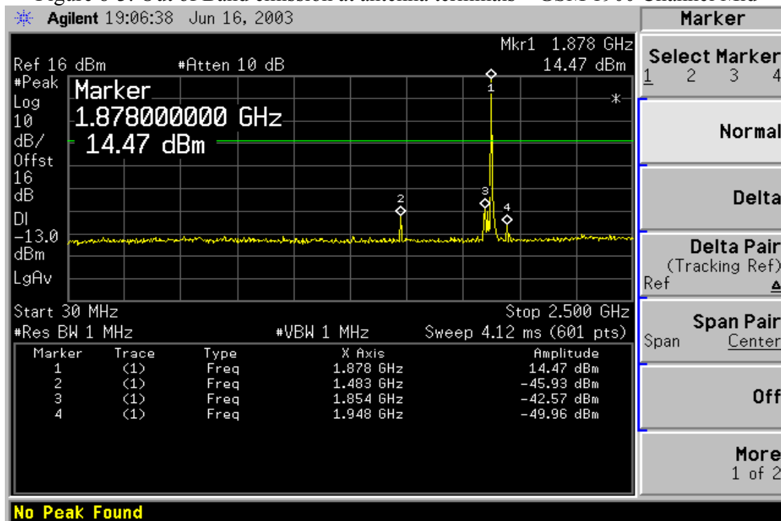
Figure 8-3: Out of Band emission at antenna terminals – GSM 1900 Channel Mid
