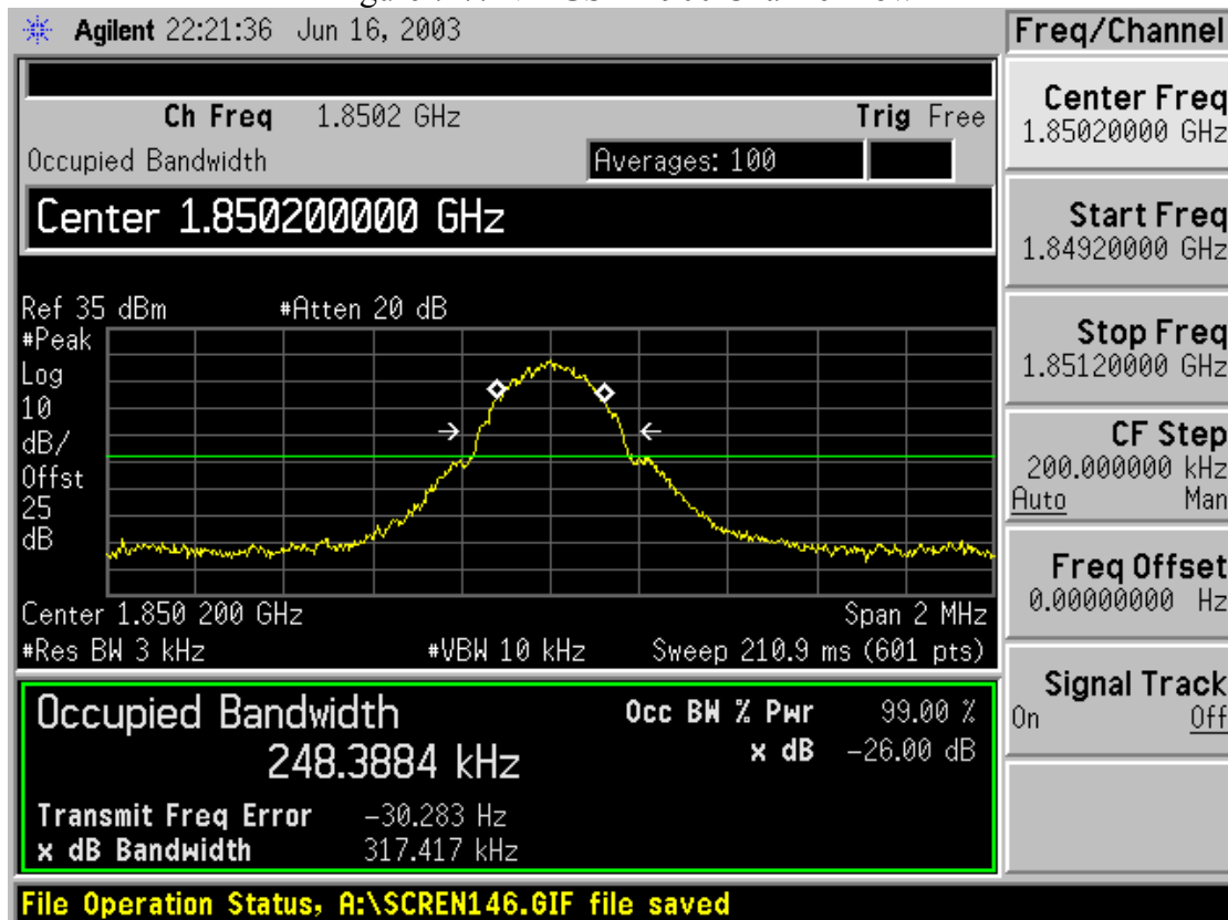
Figure 7-7: NB-GSM 1900 Channel Low
