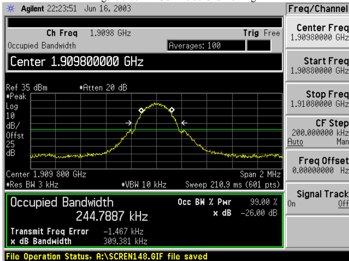
Figure 7-9: NB-GSM 1900 Channel High
