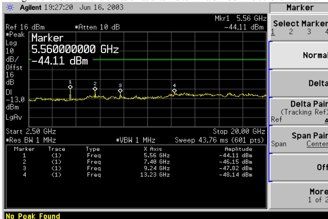
Figure 8-2: Out of Band emission at antenna terminals – GSM 1900 Channel Low
