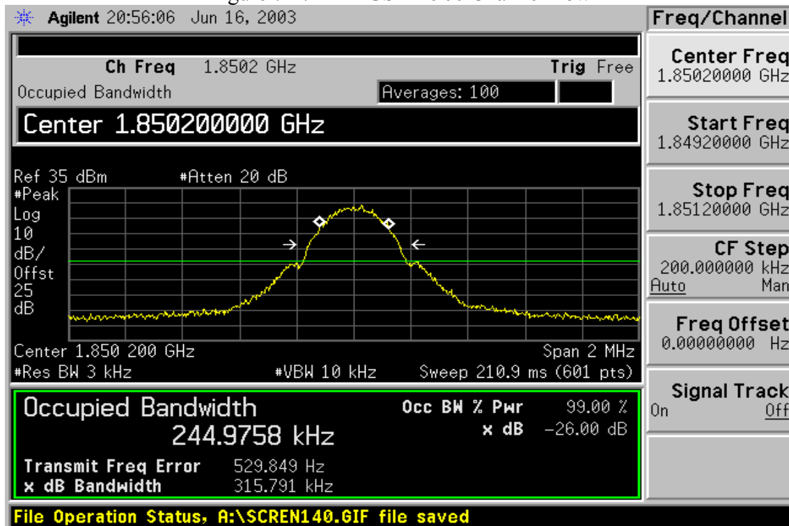
Figure 7-1: PDA-GSM 1900 Channel Low
