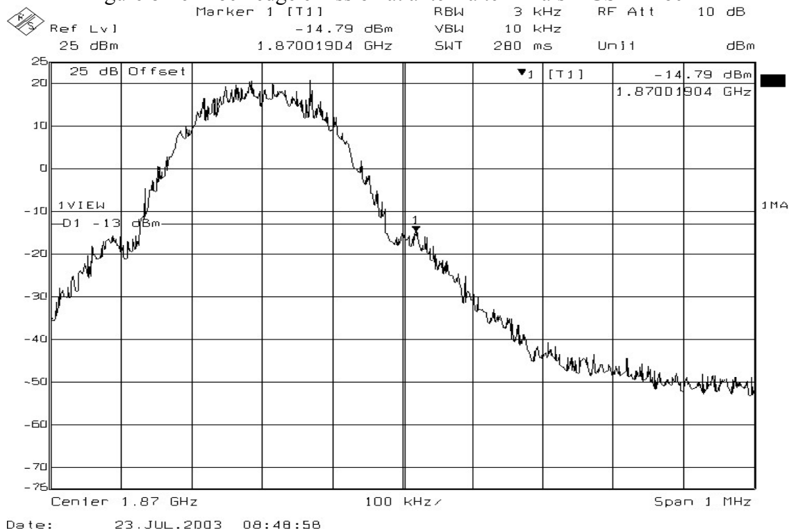
Figure 8-16 Block edge emission at antenna terminals – GSM Block D
