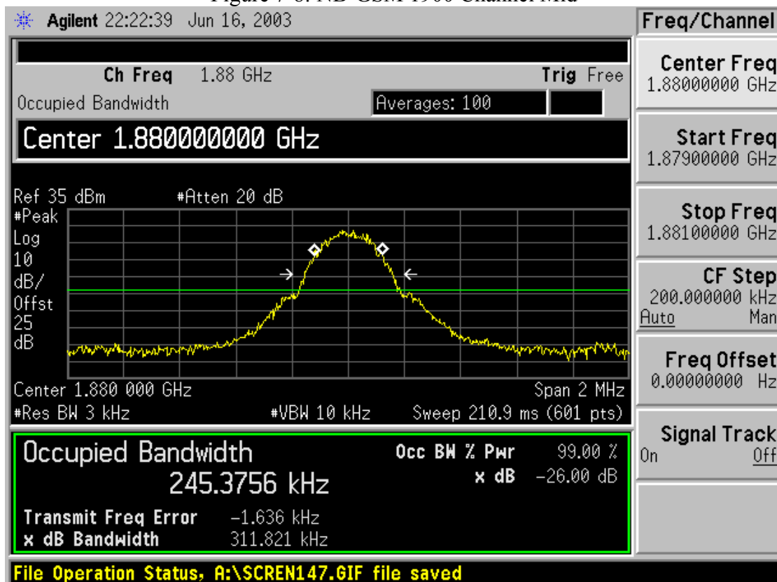
Figure 7-8: NB-GSM 1900 Channel Mid
