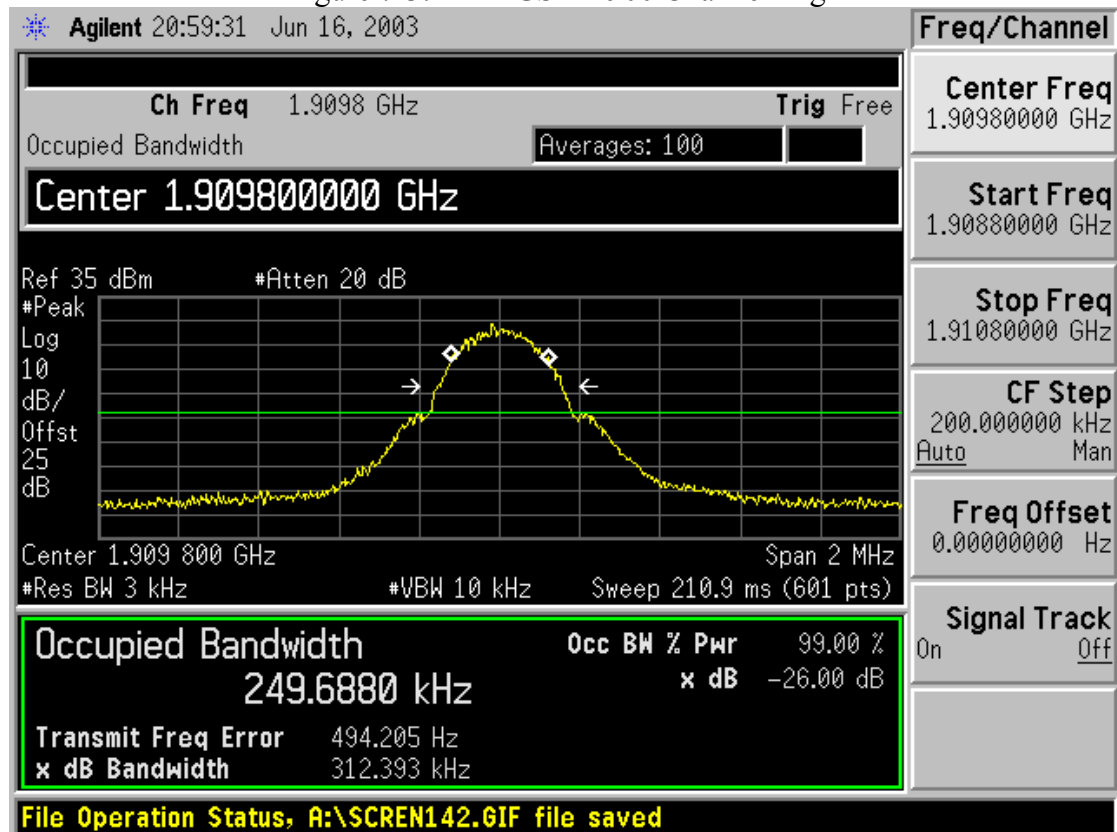
Figure 7-3: PDA-GSM 1900 Channel High
