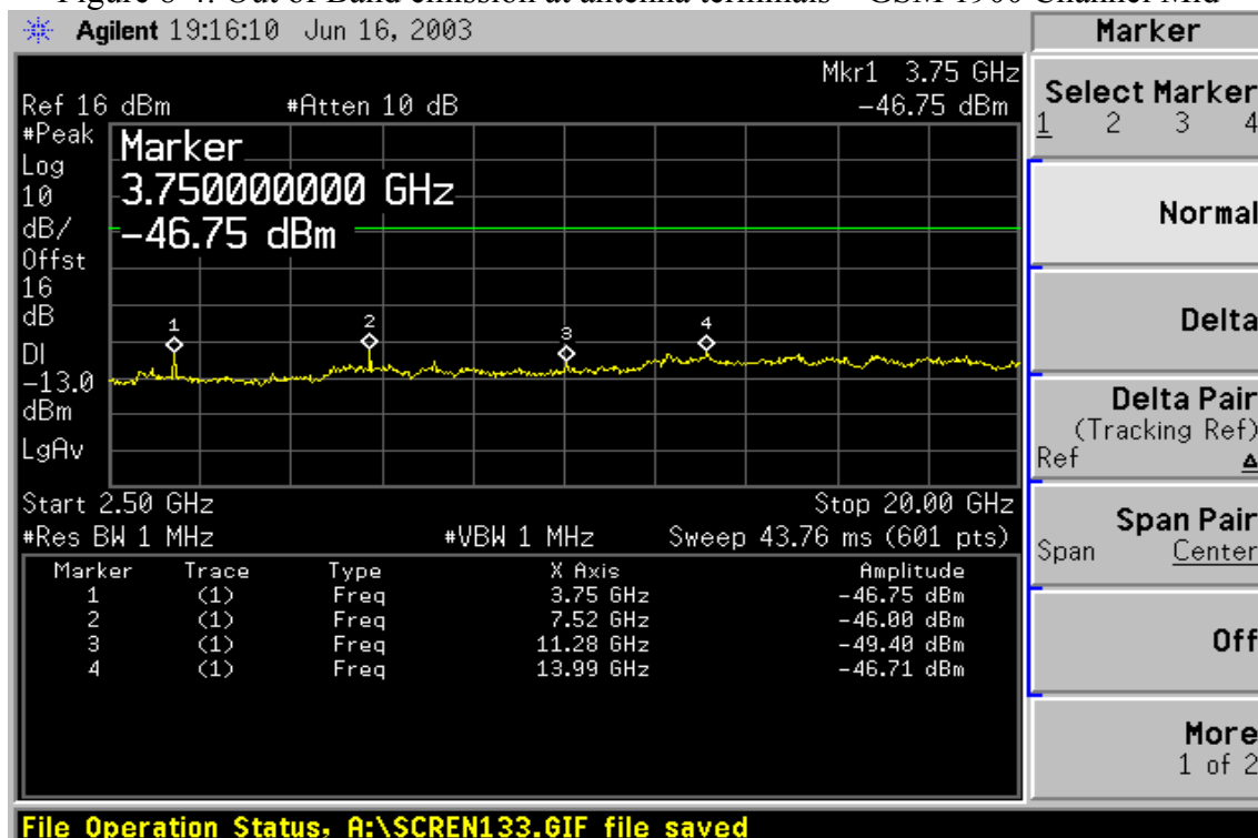
Figure 8-4: Out of Band emission at antenna terminals – GSM 1900 Channel Mid
