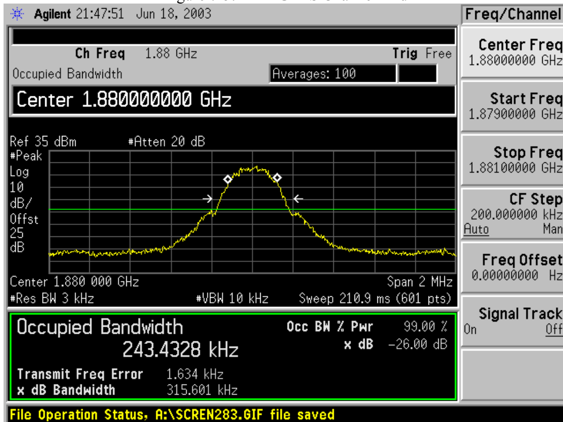
Figure 7-5: PDA-GPRS Channel Mid
