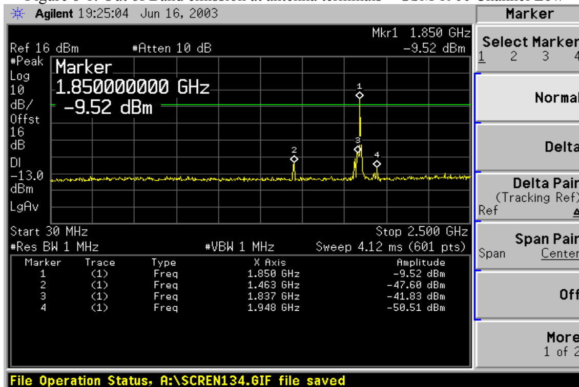
Figure 8-1: Out of Band emission at antenna terminals – GSM 1900 Channel Low
