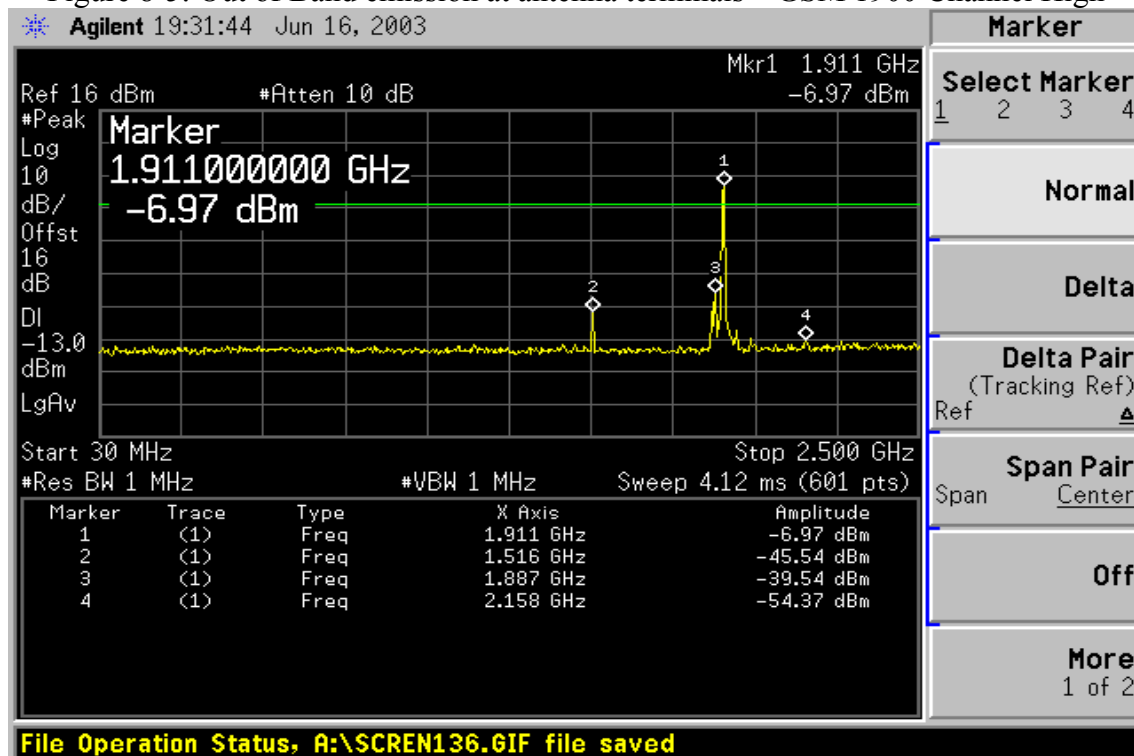
Figure 8-5: Out of Band emission at antenna terminals – GSM 1900 Channel High
