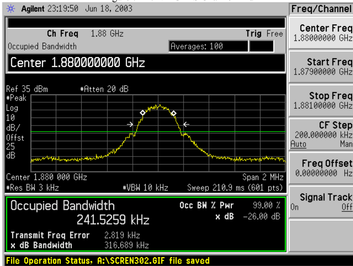
Figure 7-11: NB-GPRS Channel Mid
