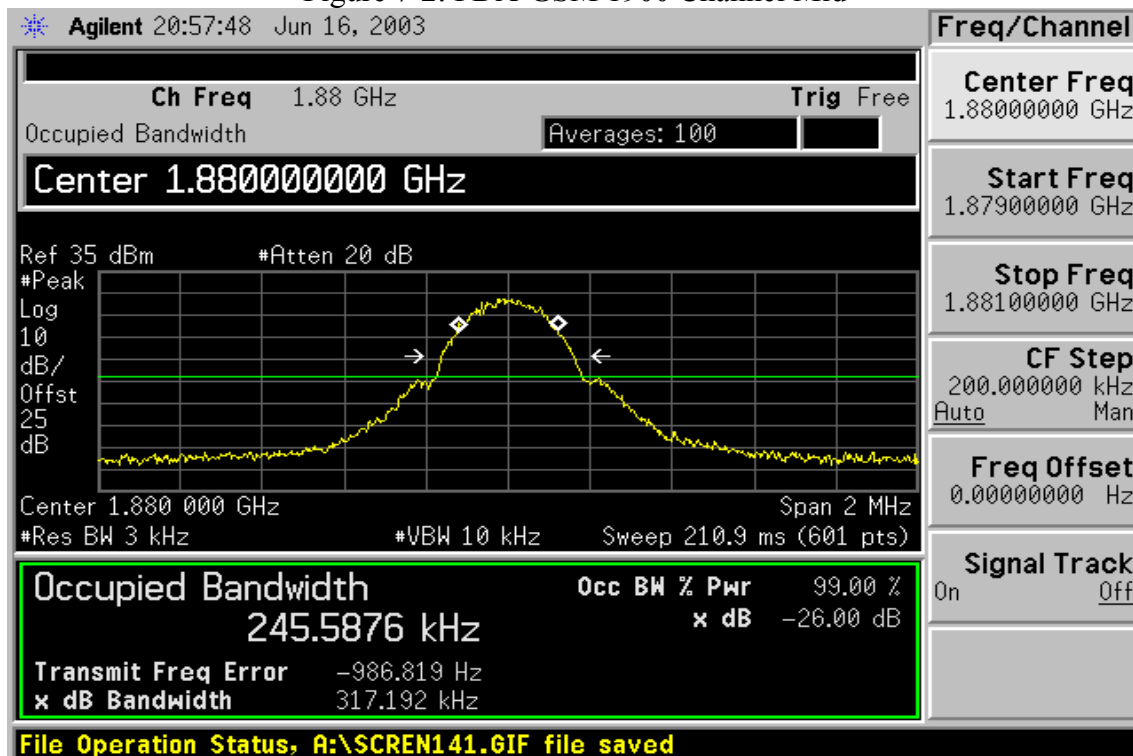
Figure 7-2: PDA-GSM 1900 Channel Mid
