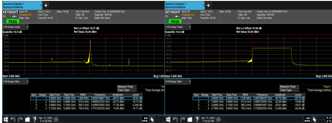
N77(50M)_CP- OFDM_QPSK_Edge_1RB_Left_Low_CH
