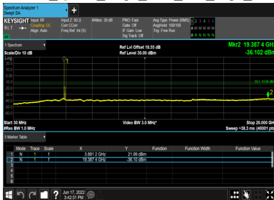
OFDM_QPSK_Edge_1RB_Left_High_CH
