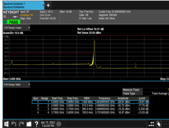
N77(100M)_CP- OFDM_QPSK_Edge_1RB_Left_Low_CH
