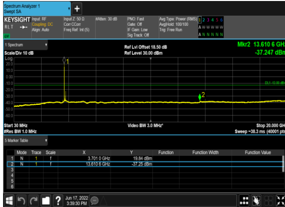
OFDM_QPSK_Edge_1RB_Left_Low_CH
