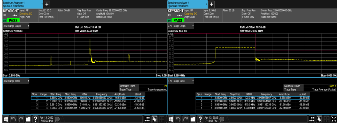
N77(50M)_CP- OFDM_QPSK_Edge_1RB_Right_High_CH
