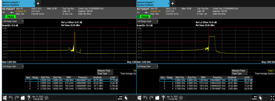
N77(10M)_CP- OFDM_QPSK_Edge_1RB_Left_Low_CH
