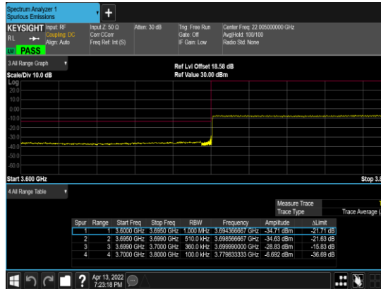
N77(100M)_CP- OFDM_QPSK_Outer_Full_Low_CH
