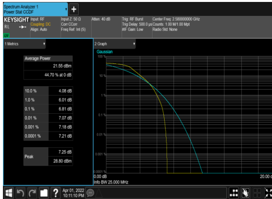
N38(20M)_DFT-s-OFDM_PI_2-BPSK_Outer_Full_Low_CH
