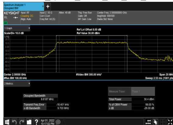
N38(10M)_DFT-s- OFDM_QPSK_Outer_Full_Mid_CH
