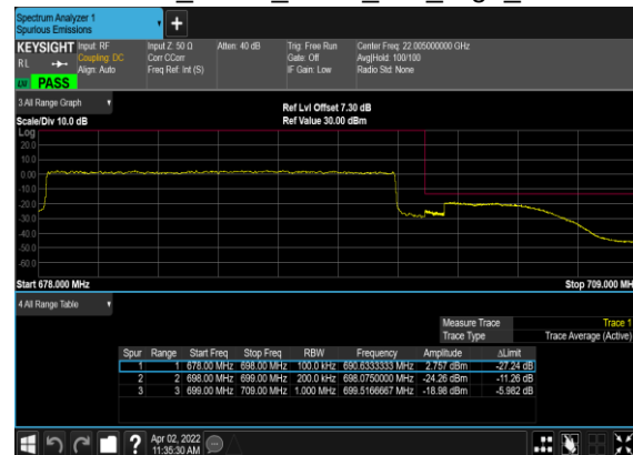
N71(20M)_DFT-s- OFDM_BPSK_Outer_Full_High_CH
