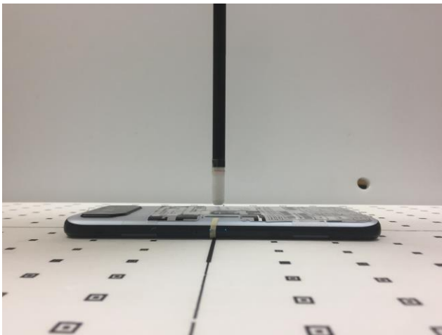
Back Side, Test Separation 2 mm
