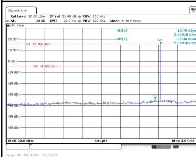
CSE Plot on CH 39 between 30 MHz ~ 3 GHz
