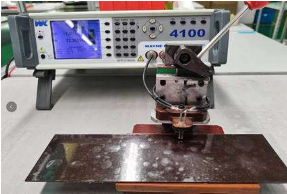
Fig4.2. NFC test environment
