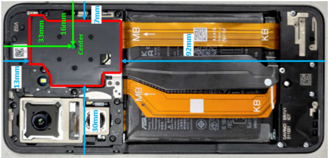
Fig4.2. NFC test environment
