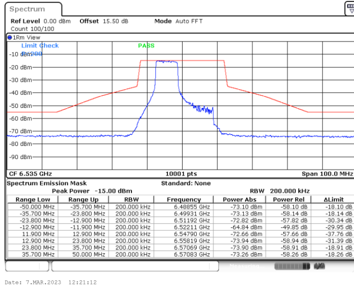
11BE20MIMO_Ant4_6535_106+26_OFDMA_1
