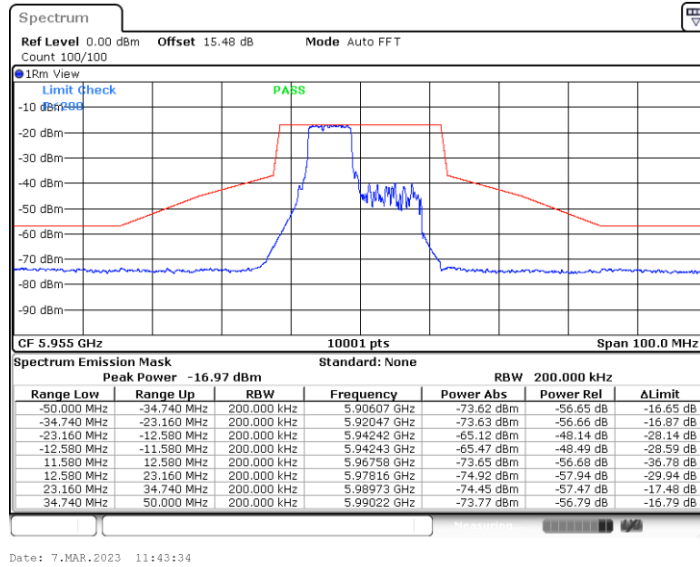
11BE20MIMO_Ant4_5955_106+26_OFDMA_1
