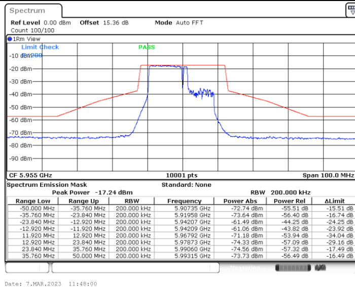
11BE20MIMO_Ant4_5955_52+26_OFDMA_1
