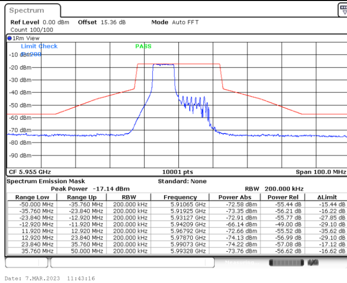
11BE20MIMO_Ant5_5955_106+26_OFDMA_1
