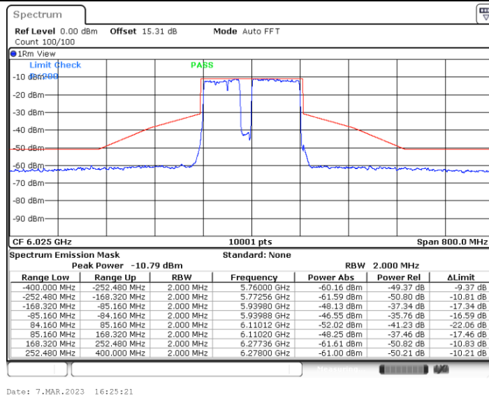
11BE160MIMO_Ant4_6025_Puncturing 20M_6
