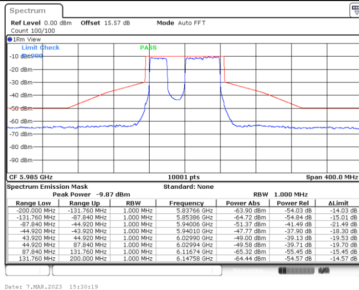
11BE80MIMO_Ant4_5985_Puncturing 20M_3
