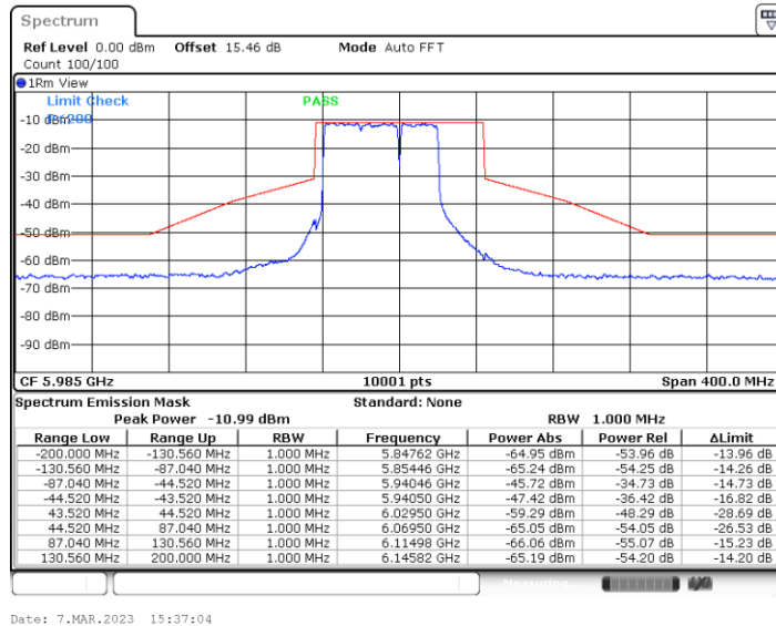
11BE80MIMO_Ant4_5985_Large RU 484+242_2
