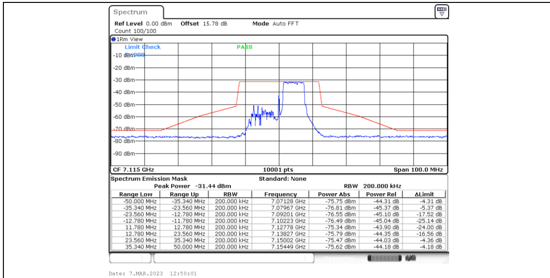
11BE20MIMO_Ant5_7115_106+26_OFDMA_2
