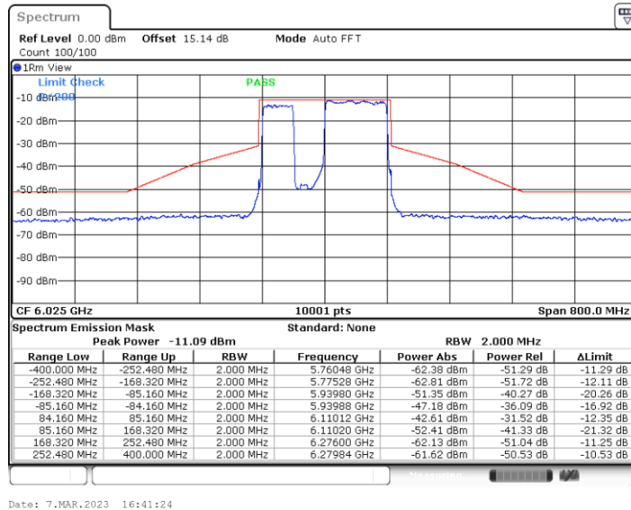
11BE160MIMO_Ant5_6025_Puncturing 40M_3
