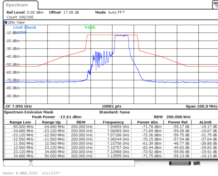
11BE20MIMO_Ant5_7095_106+26_OFDMA_2
