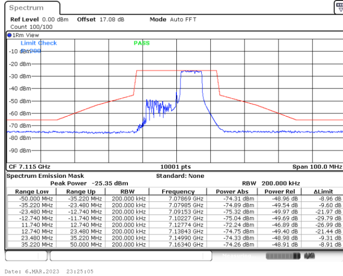
11BE20MIMO_Ant5_7115_106+26_OFDMA_2
