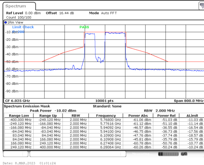
11BE160MIMO_Ant5_6025_Puncturing 40M_3
