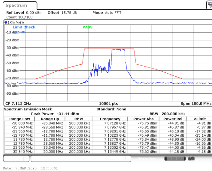
11BE20MIMO_Ant5_7115_106+26_OFDMA_2
