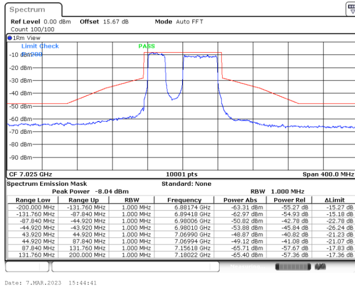
11BE80MIMO_Ant5_7025_Puncturing 20M_3
