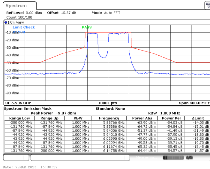
11BE80MIMO_Ant4_5985_Puncturing 20M_3
