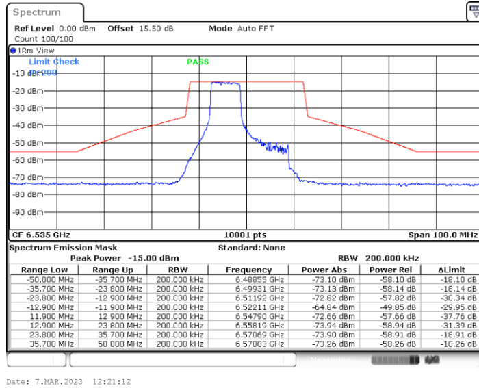
11BE20MIMO_Ant4_6535_106+26_OFDMA_1
