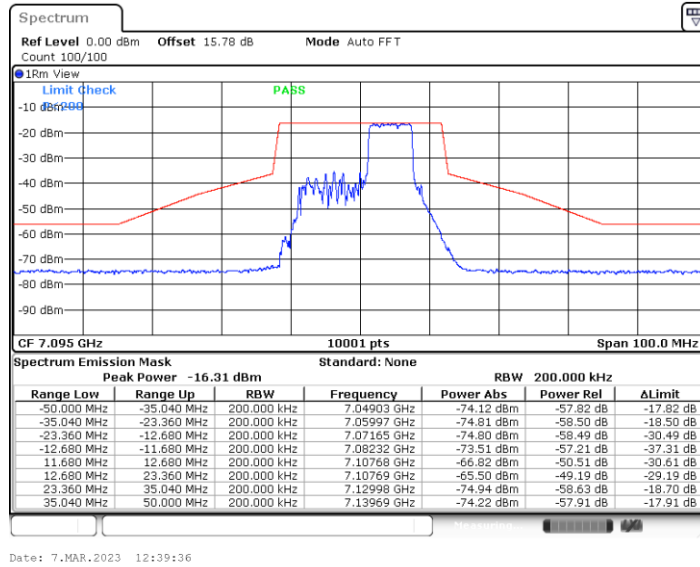
11BE20MIMO_Ant5_7095_106+26_OFDMA_2
