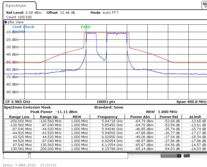
11BE80MIMO_Ant5_5985_Puncturing 20M_3
