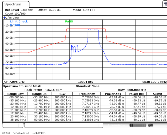
11BE20MIMO_Ant4_7095_106+26_OFDMA_2
