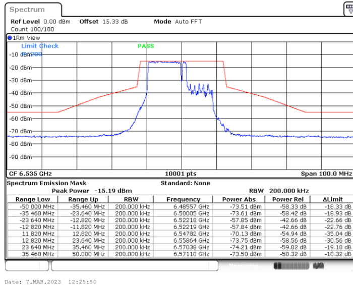
11BE20MIMO_Ant4_6535_52+26_OFDMA_1
