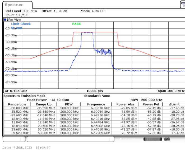
11BE20MIMO_Ant4_6435_106+26_OFDMA_1
