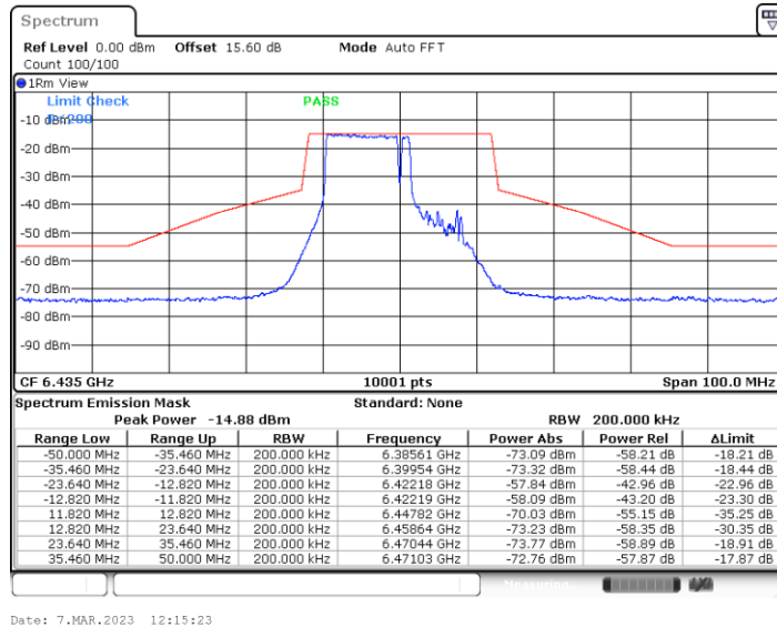
11BE20MIMO_Ant4_6435_52+26_OFDMA_1
