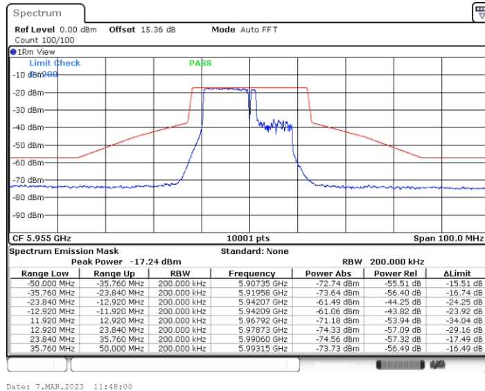
11BE20MIMO_Ant4_5955_52+26_OFDMA_1
