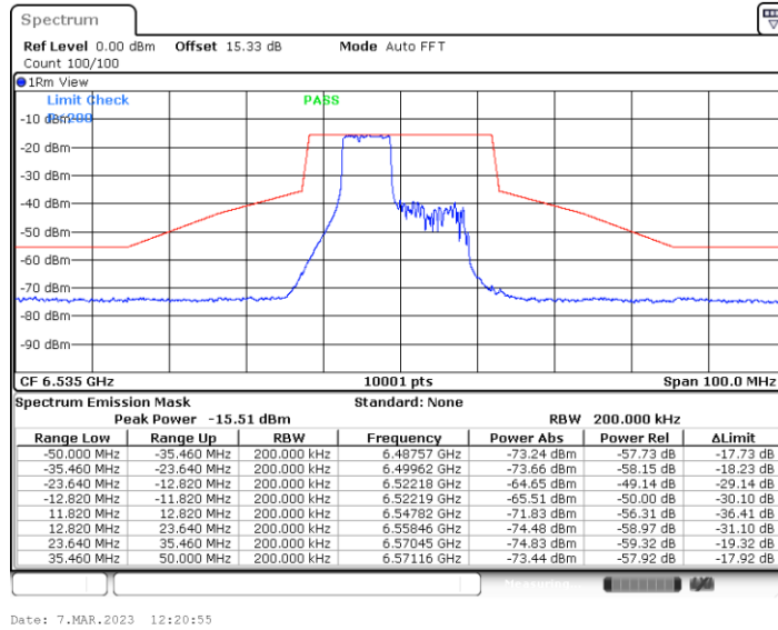
11BE20MIMO_Ant5_6535_106+26_OFDMA_1
