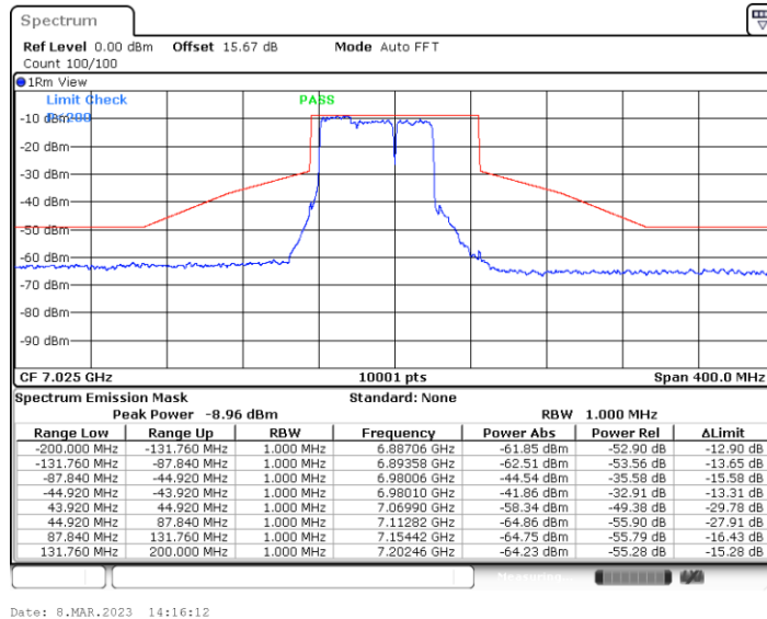
11BE80MIMO_Ant5_7025_Puncturing 20M_1
