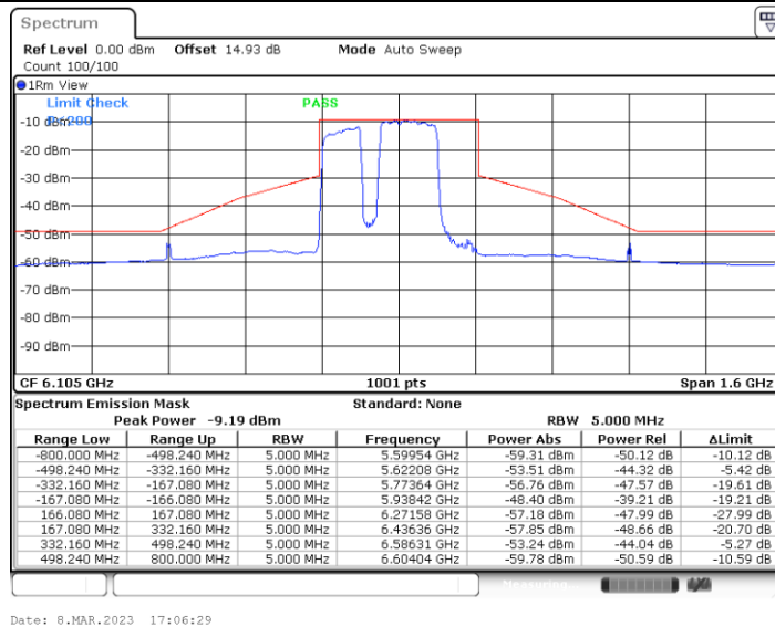
11BE320MIMO_Ant4_6105_Large RU 996*2+484_6
