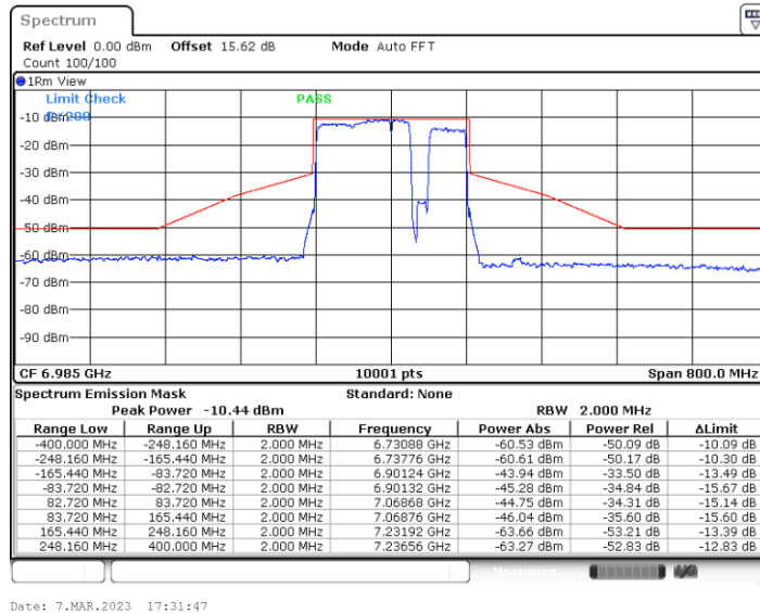
11BE160MIMO_Ant5_6985_Puncturing 20M_8
