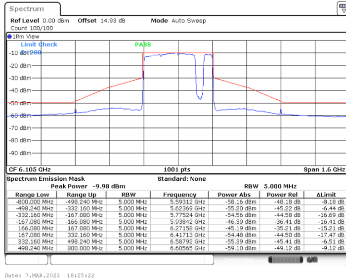
11BE320MIMO_Ant4_6105_Puncturing 40M_8
