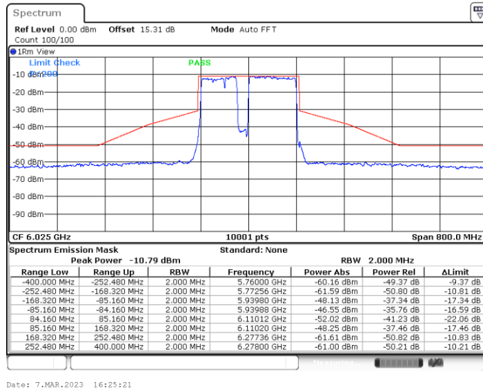
11BE160MIMO_Ant4_6025_Puncturing 20M_6
