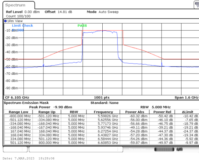
11BE320MIMO_Ant4_6105_Large RU 996*2+484_3
