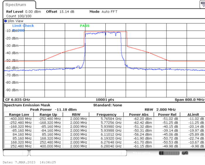
11BE160MIMO_Ant4_6025_Large RU 996+484_3
