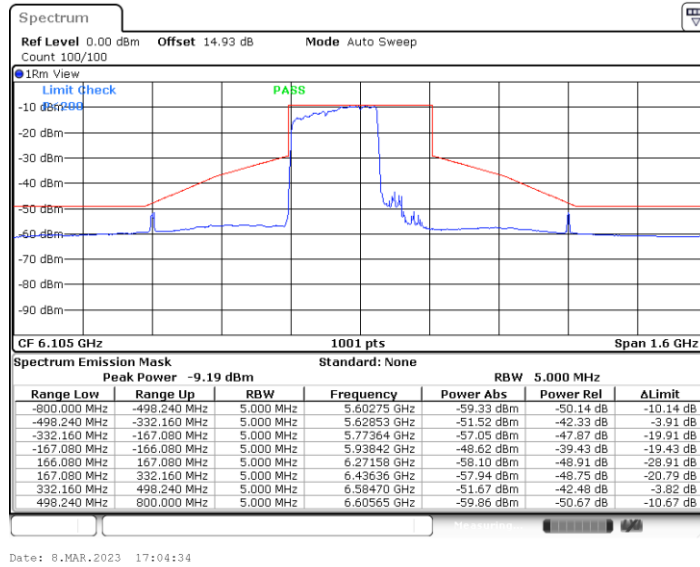
11BE320MIMO_Ant4_6105_Large RU 996*3_4
