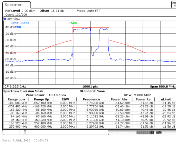
11BE160MIMO_Ant4_6025_Large RU 996+484_4
