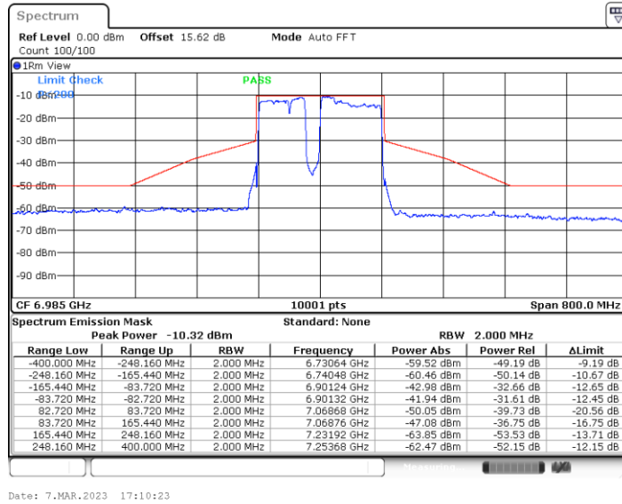
11BE160MIMO_Ant5_6985_Puncturing 20M_6
