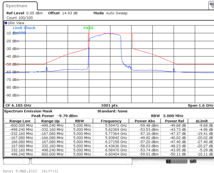
11BE320MIMO_Ant4_6105_Large RU 996*3+484_5
