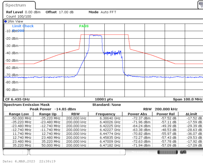
11BE20MIMO_Ant6_6435_106+26_OFDMA_1
