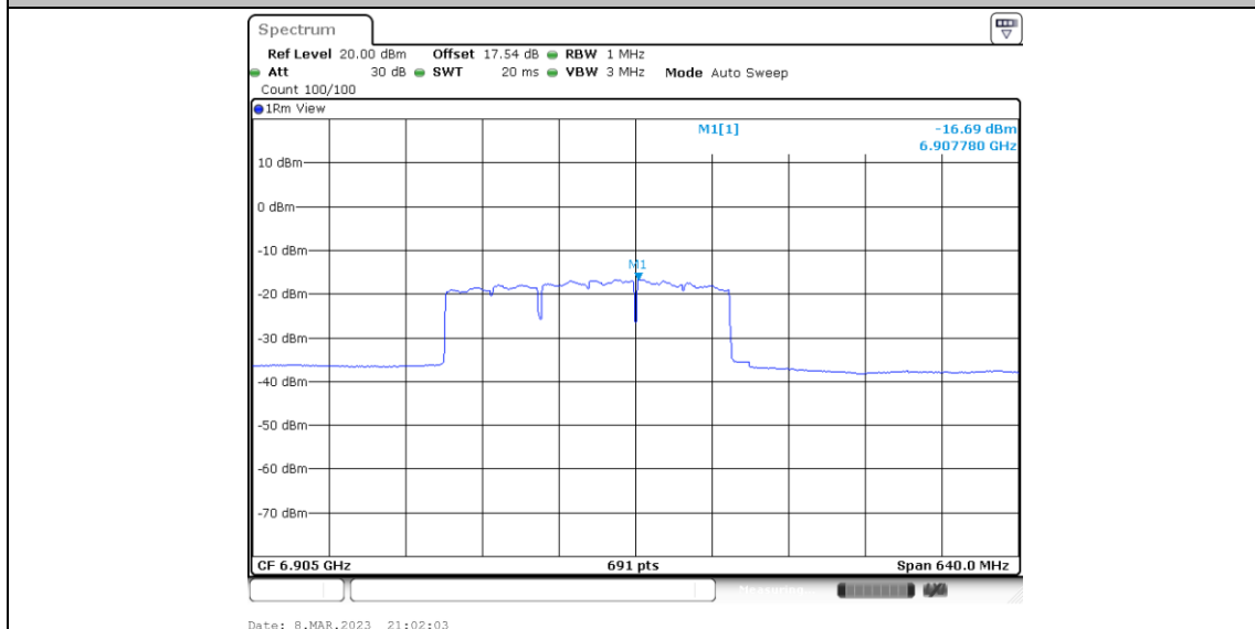
11BE320MIMO_Ant6_6905_Large RU 996*3+484_5
