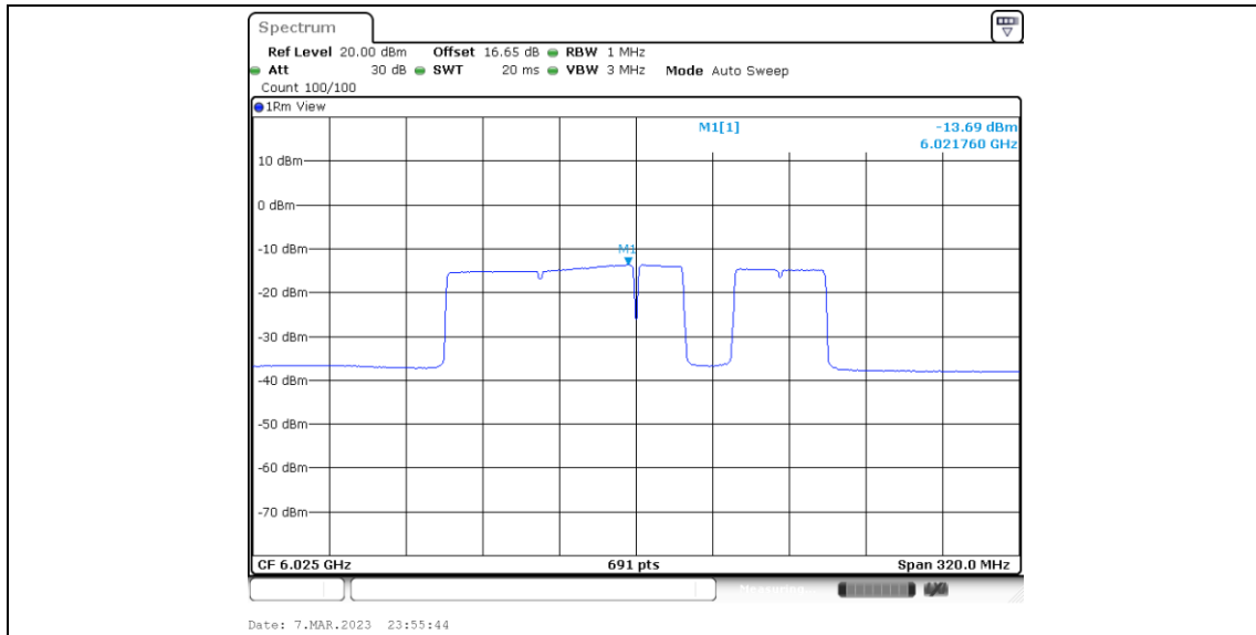
11BE160MIMO_Ant6_6025_Puncturing 20M_8
