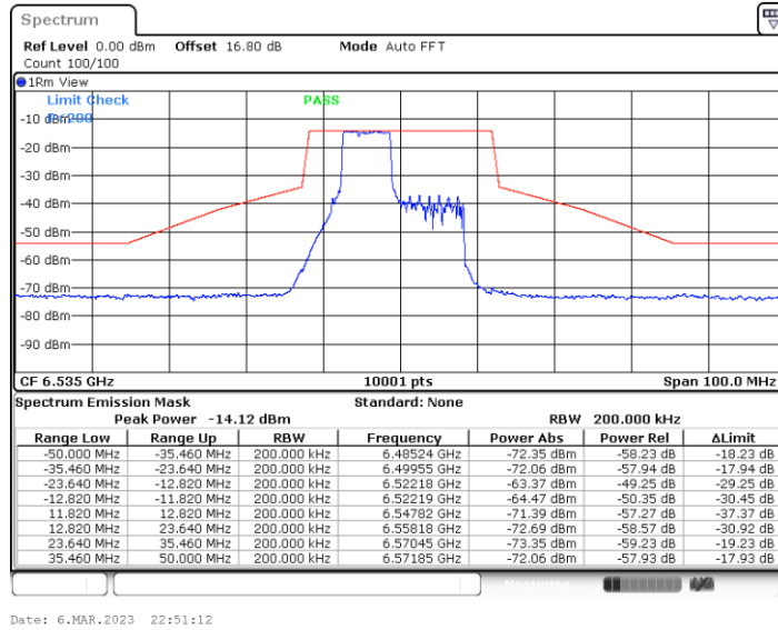
11BE20MIMO_Ant6_6535_106+26_OFDMA_1
