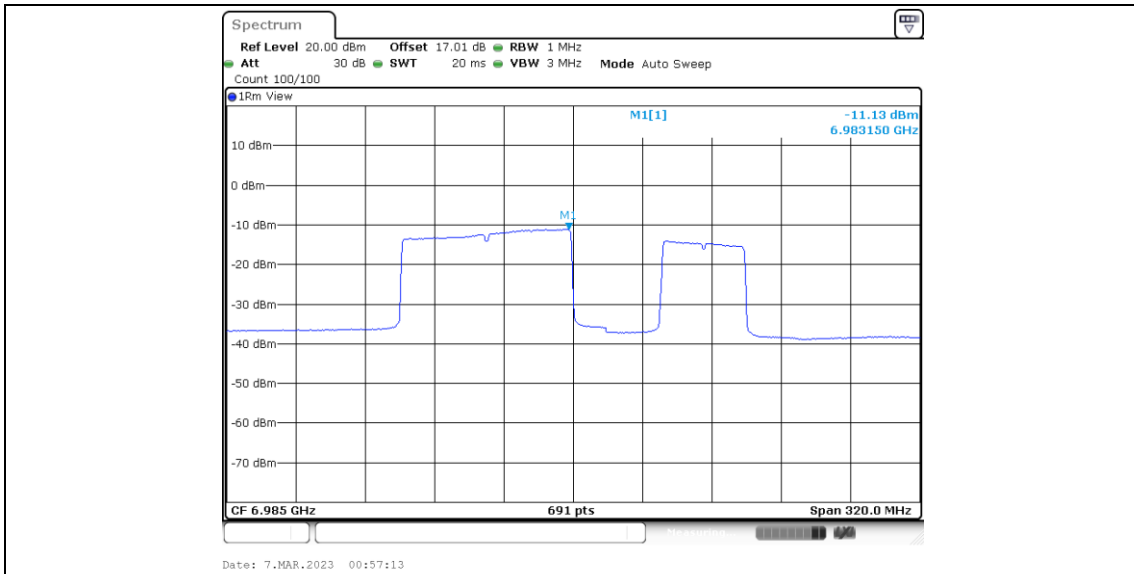
11BE160MIMO_Ant5_6985_Large RU 996+484_4
