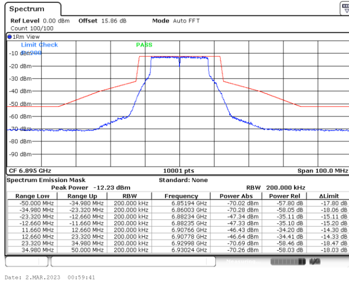
11A-CDD_Ant2_6895
