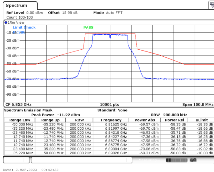
11A-CDD_Ant2_6855
