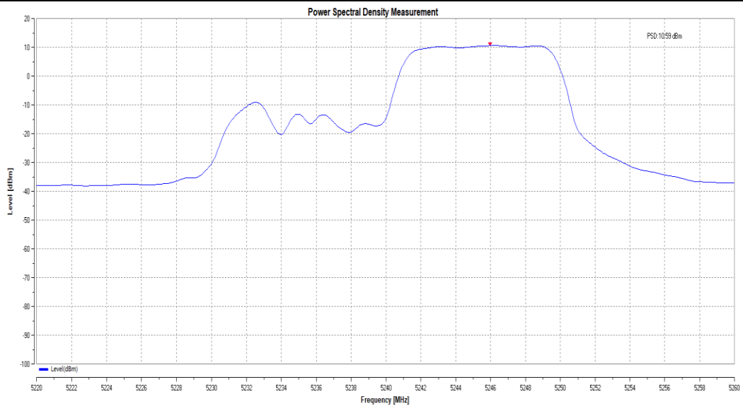
11BE20MIMO_total_5240_106Tone_RU54
