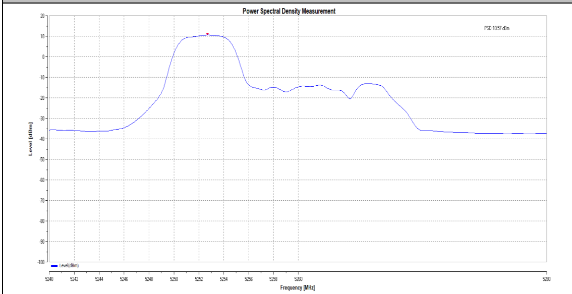
11BE20MIMO_total_5260_52Tone_RU37
