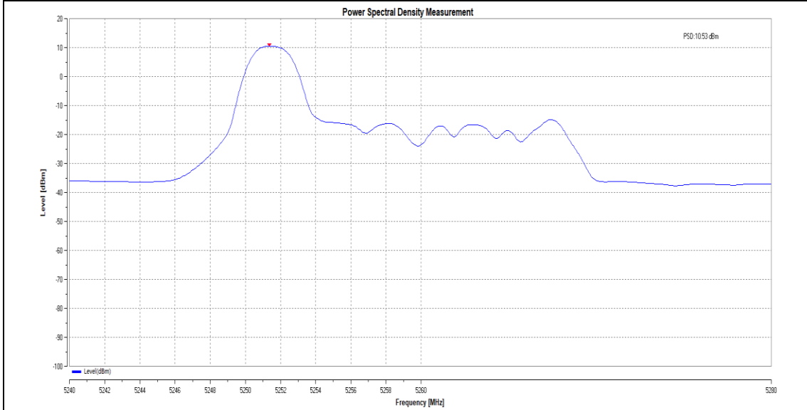
11BE20MIMO_total_5260_52Tone_RU37
