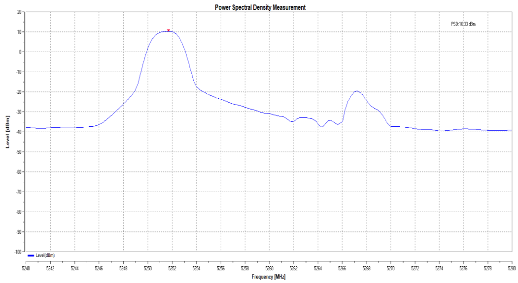
11BE20MIMO_total_5260_52Tone_RU37
