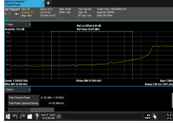
N30(5M)_DFT-s-OFDM_BPSK_Outer_Full_Low_CH_CHP_PASS
