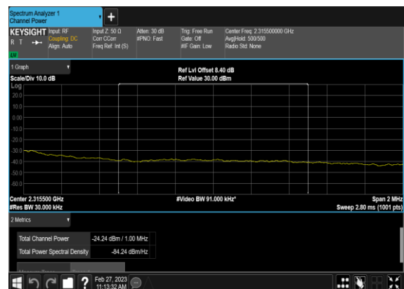
N30(10M)_DFT-s-OFDM_QPSK_Outer_Full_Low_CH_ CHP_PASS
