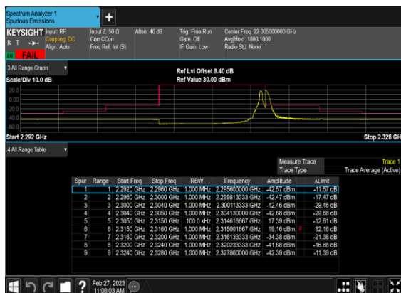
N30(10M)_DFT-s-OFDM_QPSK_Edge_1RB_Right_ t_Low_CH
