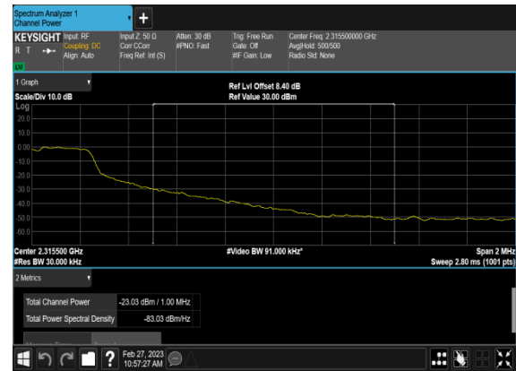
N30(5M)_DFT-s-OFDM_QPSK_Outer_Full_High_CH_ CHP_PASS
