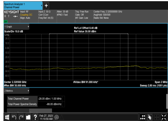
N30(10M)_DFT-s-OFDM_BPSK_Outer_Full_Low_CH_ CHP_PASS
